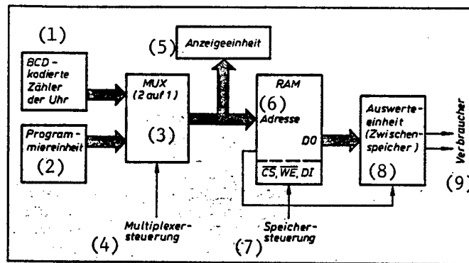
Fig. 1. Block diagram of point of time programming
