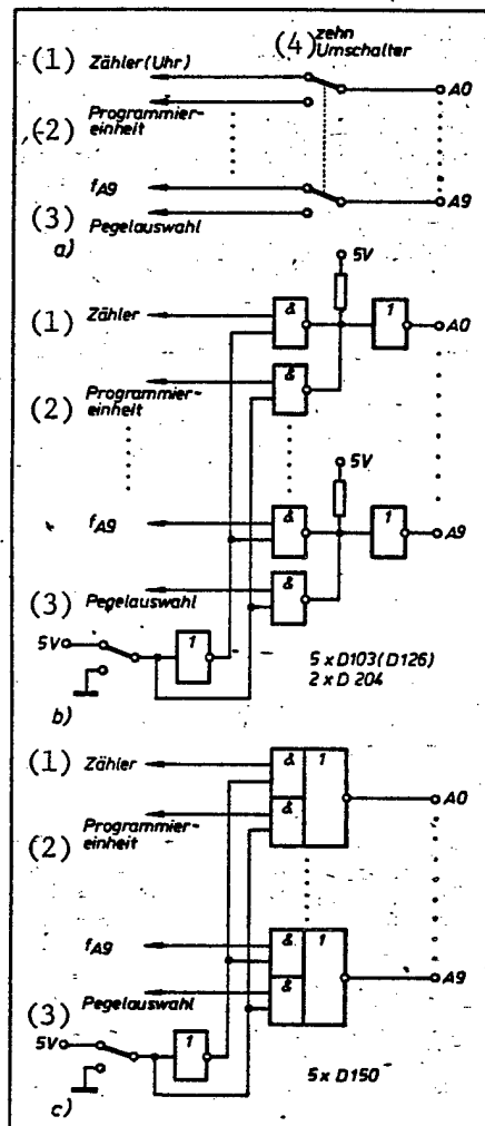
Fig. 3. Multiplexer versions
