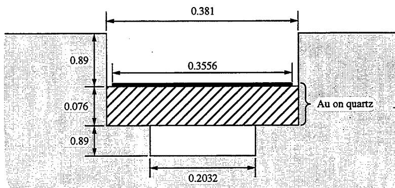
Figure 7.11 Schematic diagrams of the NRAO A2621-TR2-T12 200-290 GHz tripler block showing (a.) the block split along the partition between the block halves, (b.) a cross-section of the stripline filter channel, (c.) a cross-section through the block detailing the output waveguide transformer and device under test mounting configuration, and (d.) the configuration for the output backshort. Note that all dimensions are in millimeters.
