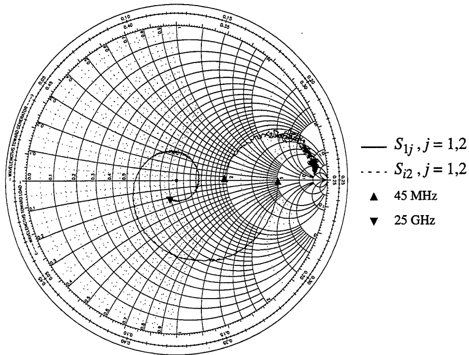
Figure 7.6 Experimental s-parameters for UVA-NRL-1174-F 75 \mu\text{m} diameter, coplanar waveguide four barrier n GaAs/ i GaAs/ i Al 0.7 Ga 0.3 As HBV test structures biased, as shown in Figure 7.3, at 10.0 V.
