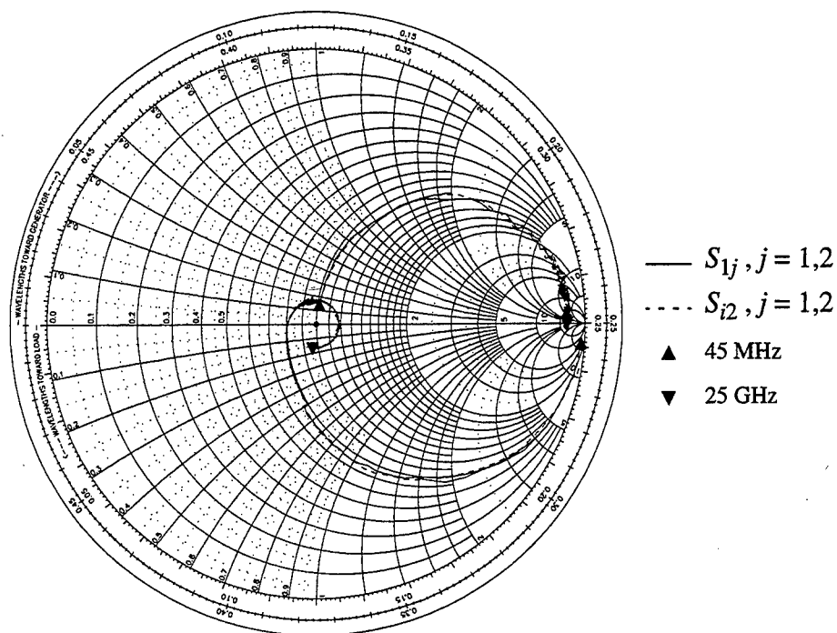
Figure 7.4 Experimental s-parameters for UVA-NRL-1174-F 75 \mu\text{m} diameter, coplanar waveguide four barrier n GaAs/ i GaAs/ i Al 0.7 Ga 0.3 As HBV test structures biased, as shown in Figure 7.3, at 0.0 V.
