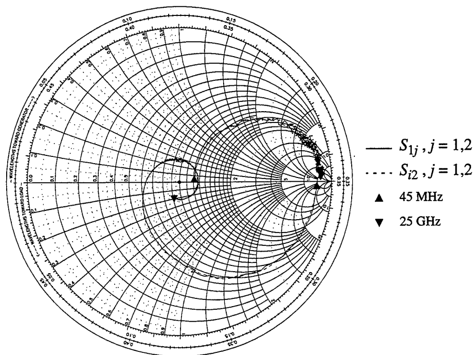
Figure 7.5 Experimental s-parameters for UVA-NRL-1174-F 75 \mu\text{m} diameter, coplanar waveguide four barrier n GaAs/ i GaAs/ i Al 0.7 Ga 0.3 As HBV test structures biased, as shown in Figure 7.3, at 5.0 V.
