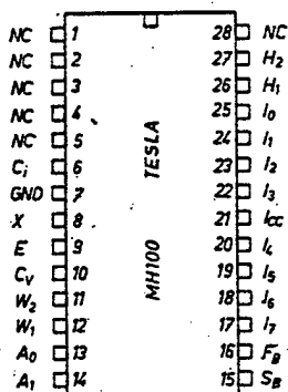
Figure 13. Wiring of casing and functions of MHL00 outlets
