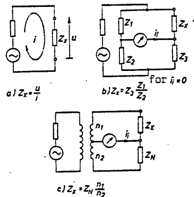
Figure 1. Basic principles of impedance measurements
