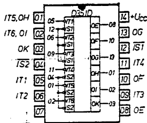
Figure 25. Schematic diagram and wiring of outlets if integrated circuits D351D, E251D
