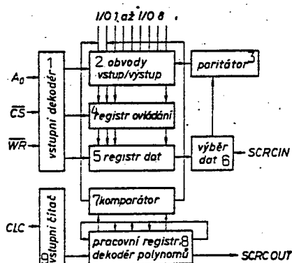
Figure 17. Functional diagram of MH101 CRC controller
