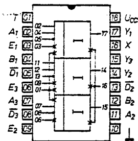
Figure 29. Schematic diagram and wiring of outlets of integrated circuit E412D
