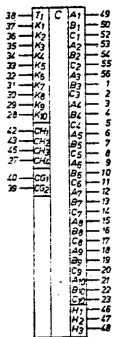
Figure 40. Schematic diagram and wiring of outlets of the U826G integrated circuit
