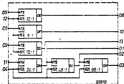
Figure 24. Functional group wiring of integrated circuits D351D, E351D
