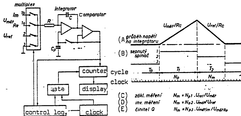
Figure 4. The "dual slope integration" method as the basis of an analog/digital converter for assessment of impedance
