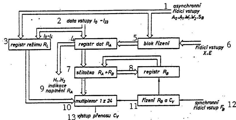
Figure 12. Functional diagram of the MHL00 circular interpolator
