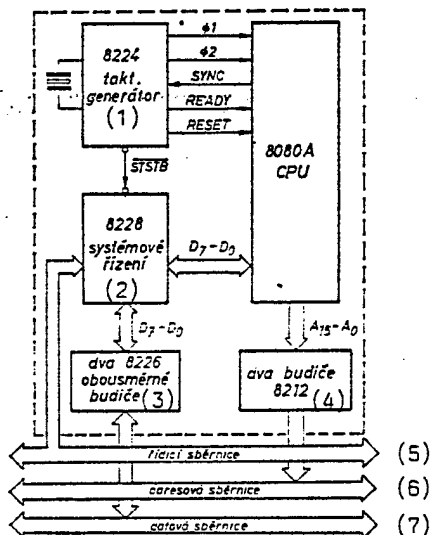
Figure 1. Complete Substitution of the 8080A System
