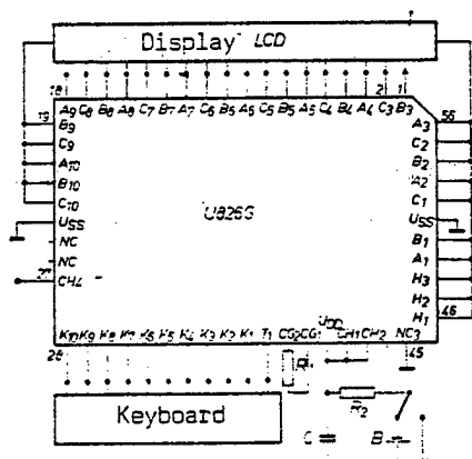
Figure 41. Recommended operational wiring of the U826G circuit in a calculator
