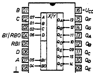
Figure 27. Schematic diagram and wiring of outlets of integrated circuits D345D, D347D
