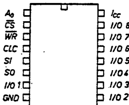
Figure 16. Wiring of casing and function of MH101 outlets
