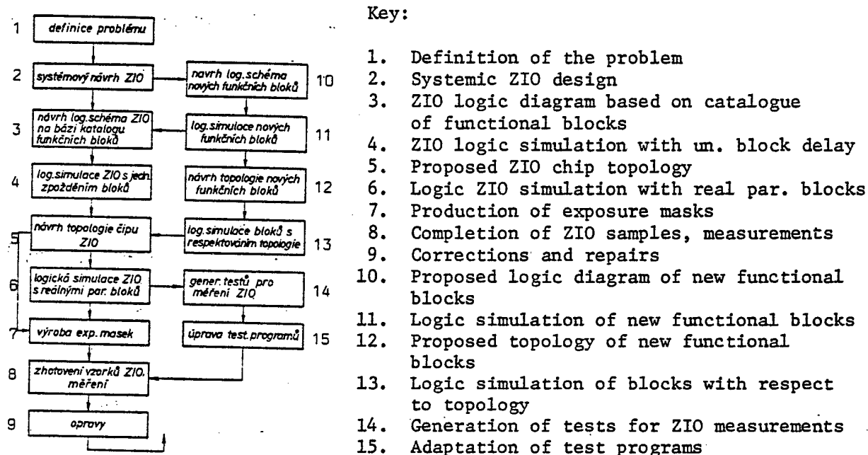
Figure 10. Sequence followed in the design of general ZIO
