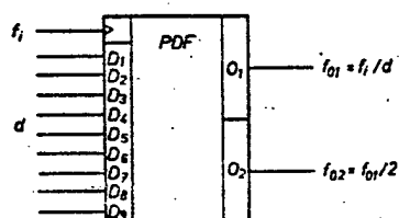
Figure 21. Equivalent diagram of programmable frequency divider
