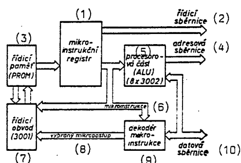
Figure 2. Simplified structure of microprogrammable processor
