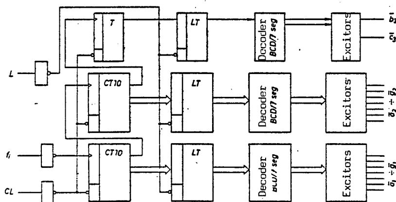
Figure 20. Functional diagram of the structure "counter-memory-decoder-excitors"
