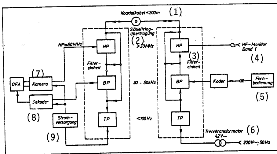
Figure 2: Block Circuit Diagram of the Underwater Television System Key:
