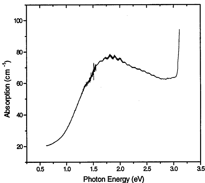
Figure 3.4-Low temperature (13K) absorption spectrum of a 6H-SiC sample contaminated with boron
