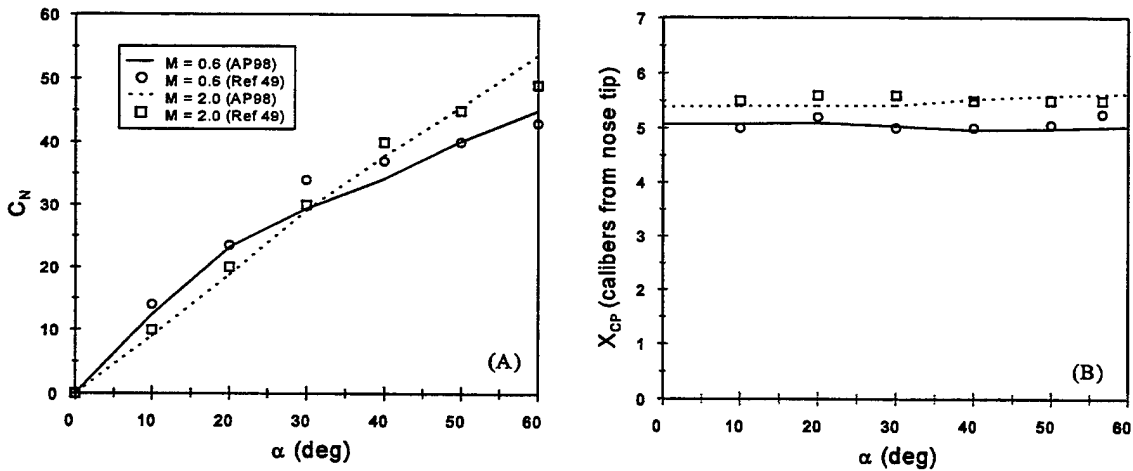
FIGURE 42. AERODYNAMIC DATA FOR THE WING-BODY CONFIGURATION OF FIGURE 41 WITH A 2:1 ELLIPTICAL CROSS SECTION BODY: (A) NORMAL FORCE COEFFICIENT, (B) CENTER OF PRESSURE
