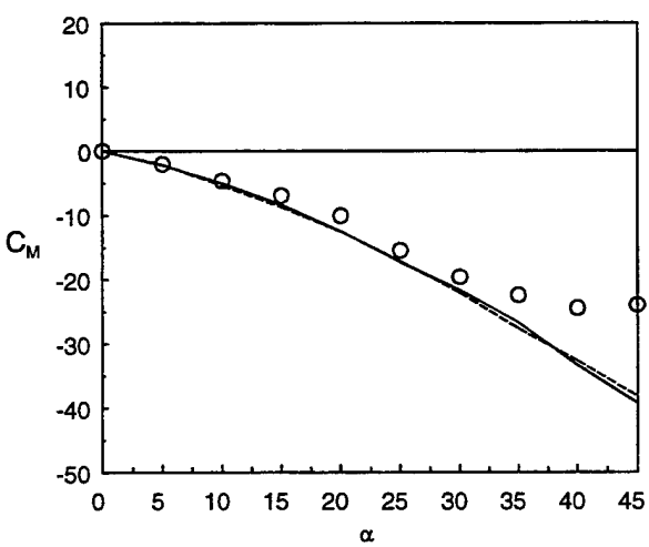
(C) M = 2.87, \delta_w = 0^\circ, \phi = 0^\circ
