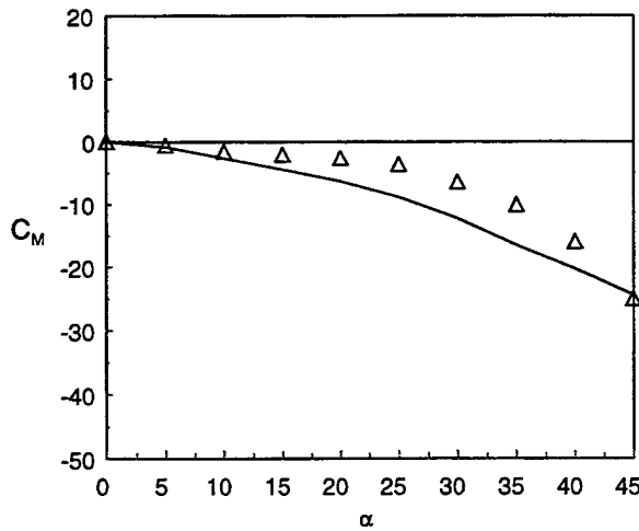
(K) M = 4.6, \delta_w = 0^\circ, \phi = 45^\circ
