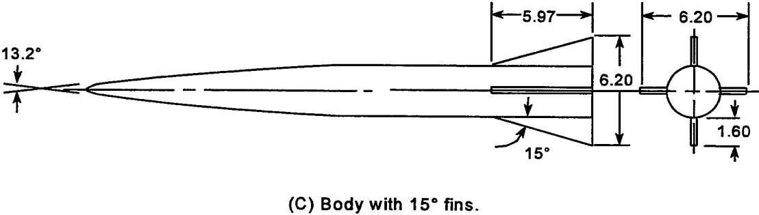
FIGURE 29. SOME CONFIGURATIONS TESTED AT M = 2.01 (REFERENCE 62)
