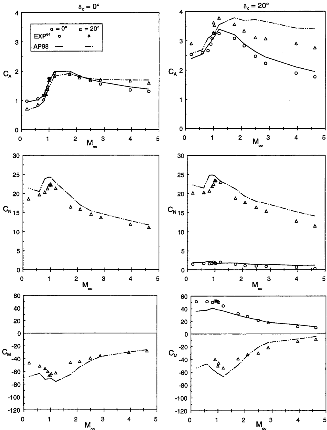
FIGURE 32C. C_A , C_N AND C_M VERSUS MACH NUMBER FOR CONFIGURATION OF FIGURE 32A ( \Phi = 45 DEG)
