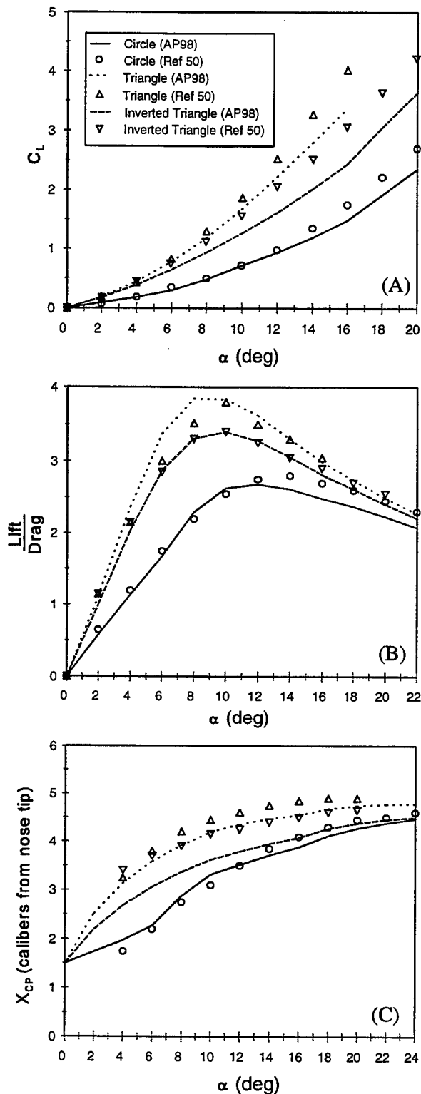
FIGURE 40. AERODYNAMIC DATA OF TRIANGLES ( k = 0.0 ) AND INVERTED TRIANGLES ( k = 0.0 ) OF FIGURE 35 COMPARED TO CIRCULAR BODY AT M = 1.98 ( \ell/d = 10 ): (A) LIFT COEFFICIENT, (B) LIFT TO DRAG RATIO, (C) CENTER OF PRESSURE
