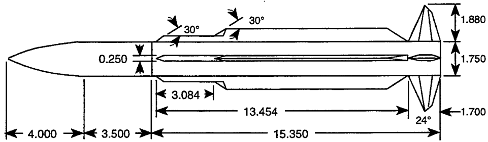
CONFIGURATION TESTED IN WIND TUNNEL (From Ref. 58) (ALL DIMENSIONS IN INCHES)
