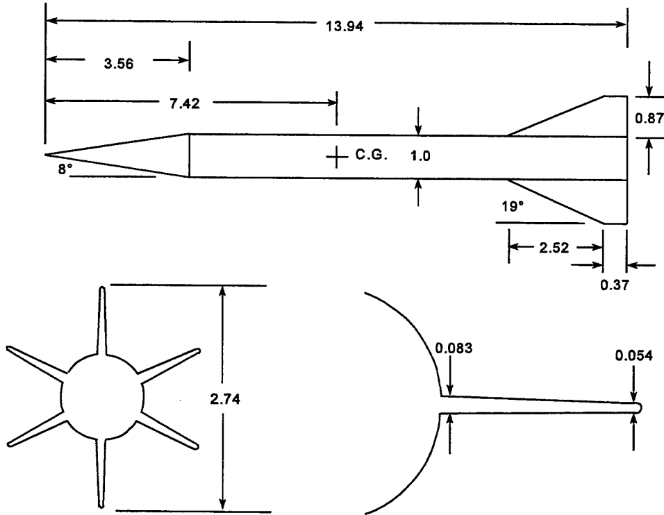
FIGURE 33A. FINNED PROJECTILE MODEL (ALL DIMENSIONS ARE IN CALIBERS, 1 CALIBER = 35.2 MM)
