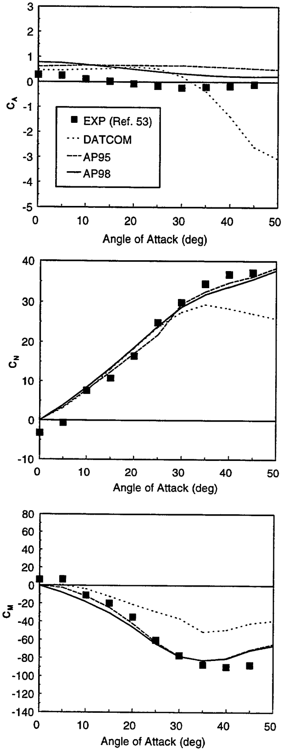
FIGURE 21C. COMPARISON OF STATIC AERODYNAMICS BETWEEN EXPERIMENT AND THEORY FOR FIGURE 21A CONFIGURATION ( \delta = 0 DEG, \Phi = 0 DEG, M_\infty = 0.2 )
