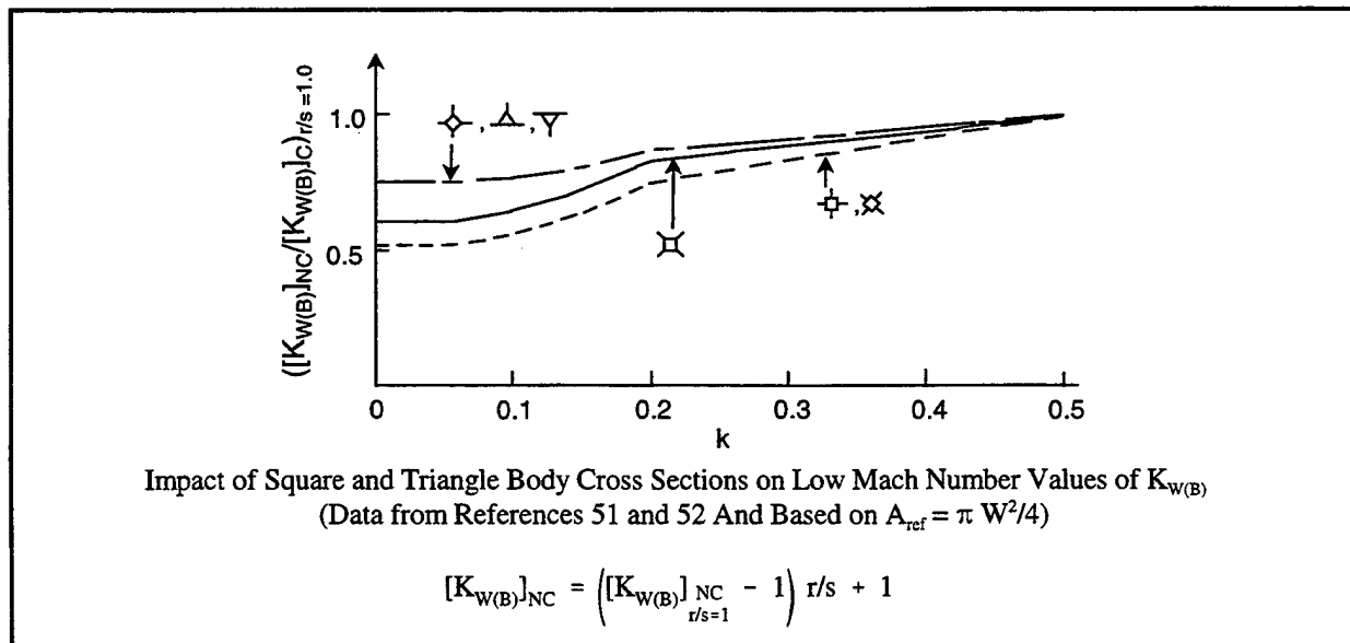
FIGURE 16. WING-BODY INTERFERENCE FACTORS (LOW AOA)
