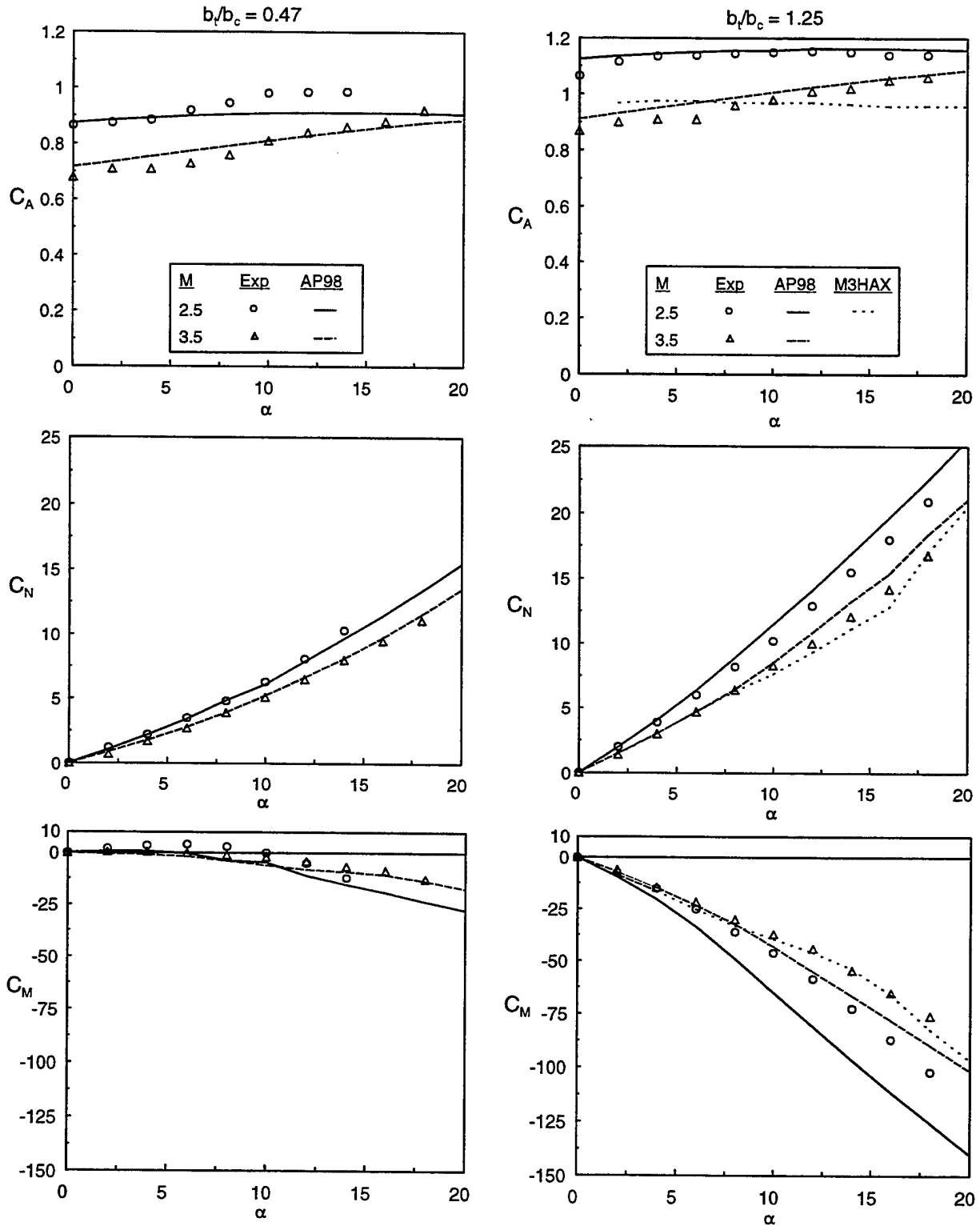
FIGURE 24. COMPARISON OF THEORY AND EXPERIMENT 56 FOR CONFIGURATIONS OF FIGURE 23 ( \Phi = 45 DEG)
