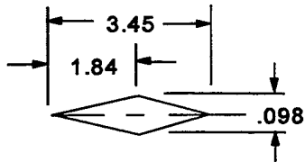
Canard Root Chord Profile
