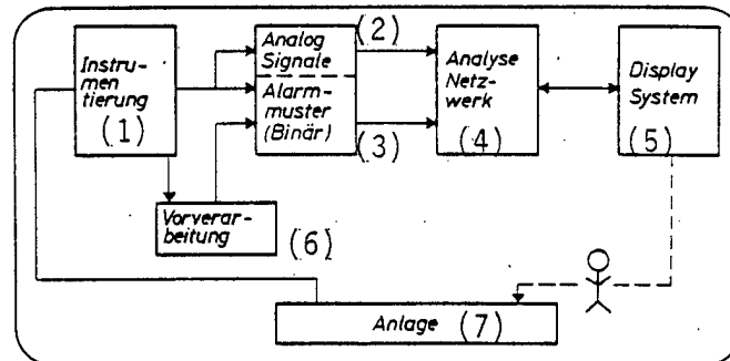
Figure 4: Schema of a Real-time Diagnostic System /1/
