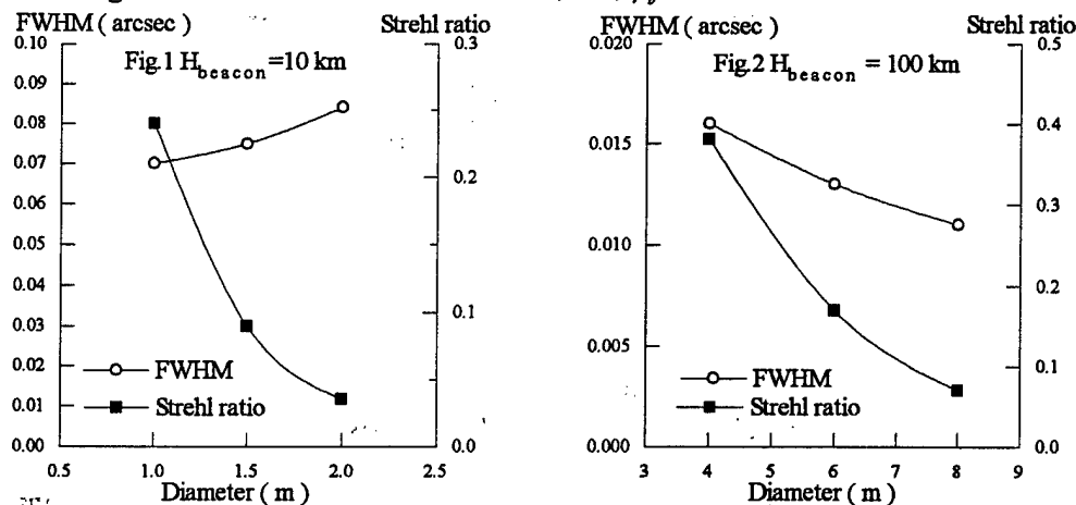
Figure 1 gives the results of calculations for the height of the reference source H_{\text{beacon}} = L = 10 \text{ km} (Rayleigh scattering), Fig.2 gives the results of calculations for the height H_{\text{beacon}} = L = 100 \text{ km} . It is assumed that the adaptive system has an infinite spatial-temporal resolution. In both cases the Strehl ratio decreases with the telescope diameter increase. At the same time the angular resolution (FWHM) varies slightly ( L = 10 \text{ km} ) and even is improved ( L = 100 \text{ km} ) remaining close to a diffraction one.
