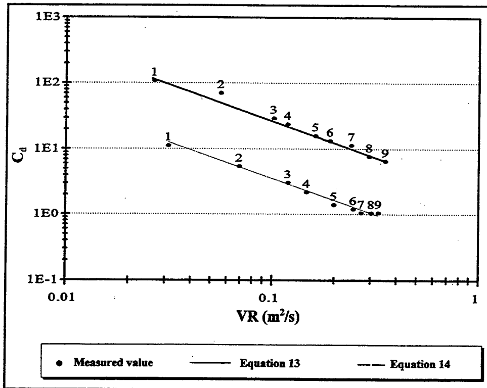
Figure 13. C_d as a function of VR plotted on log-log scale for conditions with debris and without leaves (Equation 13) and without debris and with leaves (Equation 14)
