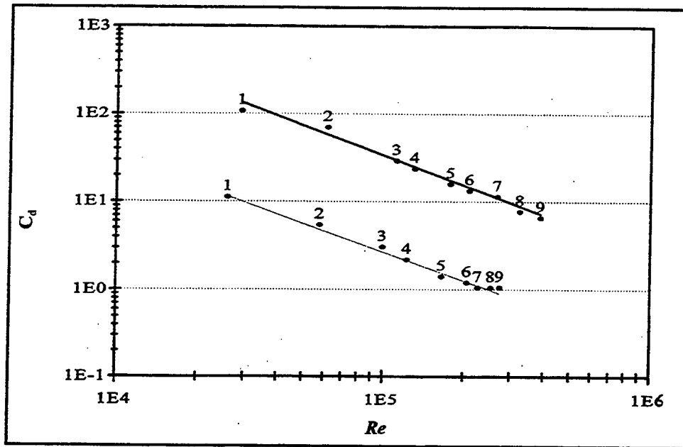
Figure 14. C_d as a function of Re plotted on log-log scale for conditions with debris and without leaves (Equation 15) and without debris and with leaves (Equation 16)
