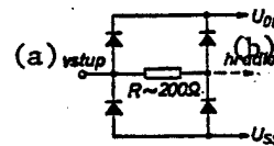
Fig. 6. Connection of protective diodes at inputs of CMOS circuits: new design
