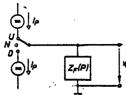
Fig. 3. Charge-pump circuit model
