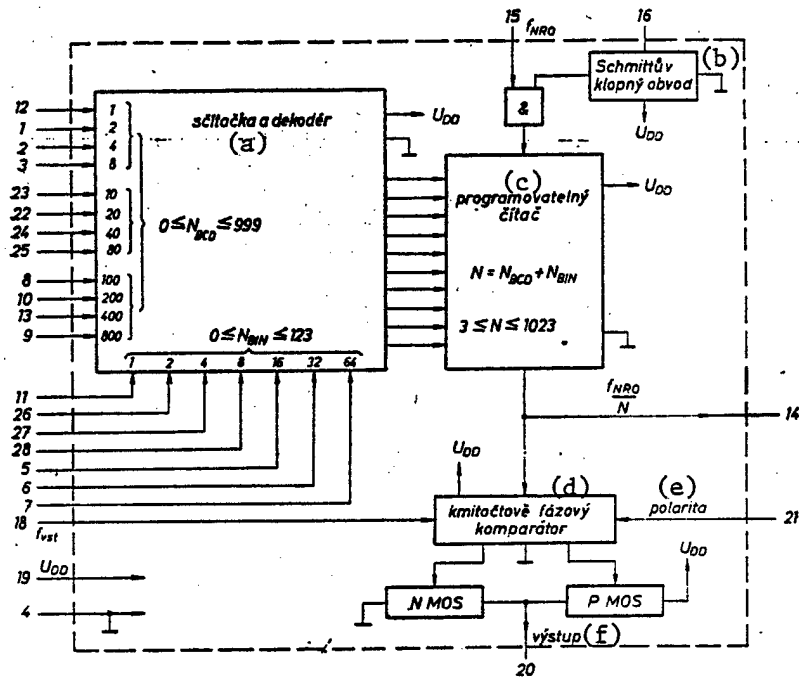
Fig. 8. Block diagram of HCTR0320 circuit
