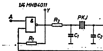
Fig. 9b. Circuit of crystal-controlled oscillator; R_1 = 1 \text{ Mohm} , R_2 = 2.2 \text{ kohm} , C_1 = 100 \text{ pH} , C_2 = 25 \text{ pF} , \text{PKJ} = 4 \text{ MHz}
