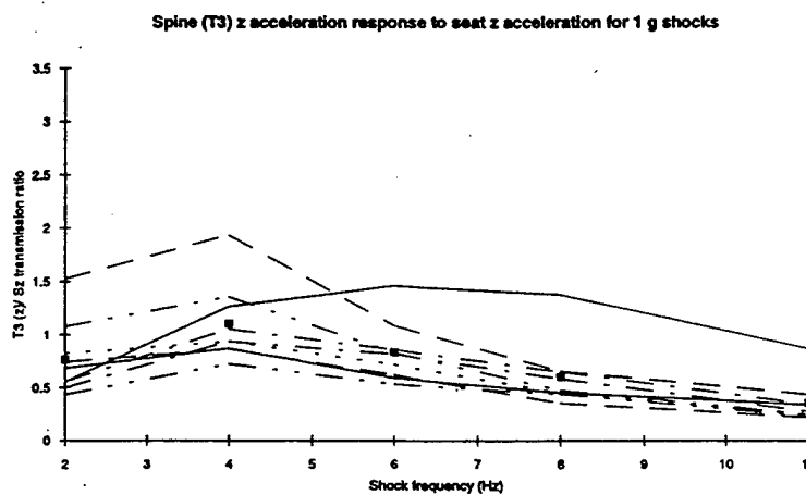
Figure 12: (a,b,c) Spine (T3) z acceleration response to seat z acceleration for 3, 2, & 1 g shocks
