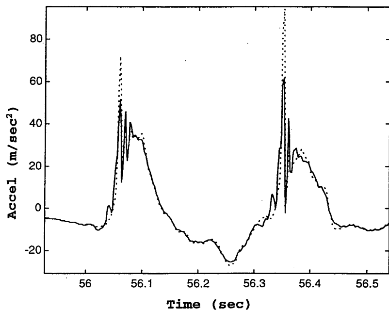
Figure 23. Recorded L4 accelerometer response to a -4 g, z axis shock at the seat and the predicted acceleration at the spinous process after correction by the skin transfer function. Dotted line = recorded L4 response; Solid line = corrected response.
