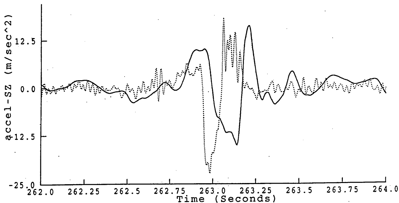
Figure 16. Abdominal respitrace displacement for a -3 g, 4 Hz z axis shock. Dotted line: seat Sz acceleration; full line: abdominal displacement.
