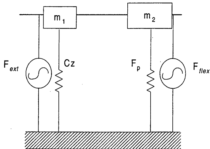
Figure 47. The eccentric segregated mass model (ESMM).
