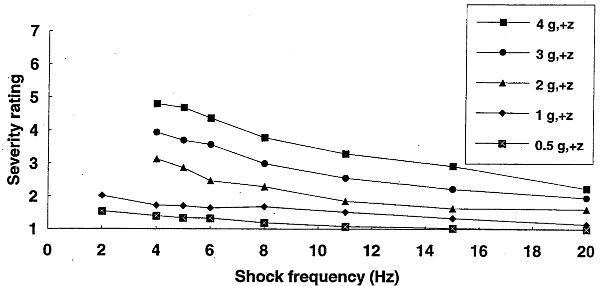
Figure 42. Subjective severity ratings to single shocks in the positive z axis as a function of shock frequency and amplitude.
