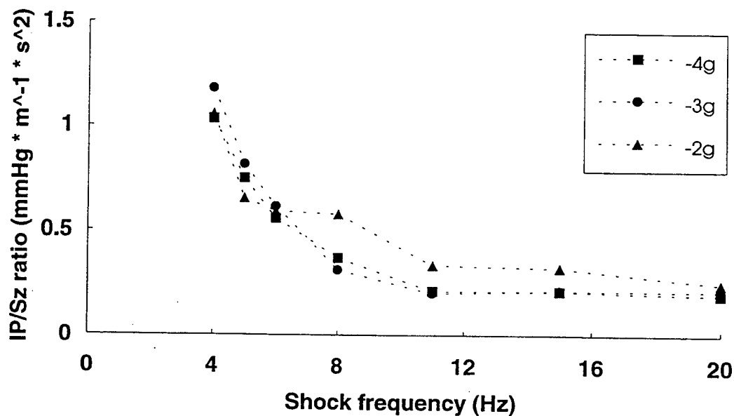
Figure 41. Second internal pressure response to seat z acceleration for negative 2, 3 and 4 g shocks.
