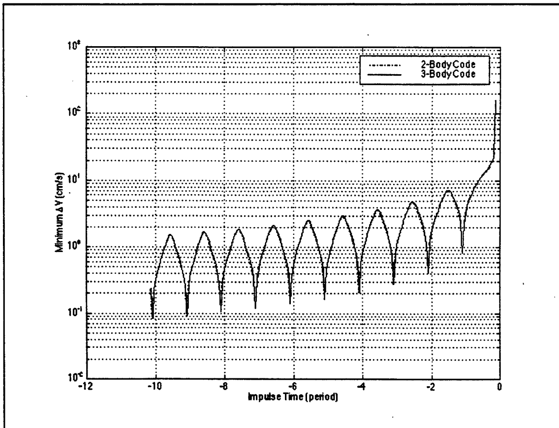
Figure 5.5 Minimum \Delta V for 1 R_{\oplus} Separation ( e=0.9 , a=1.05 AU)
