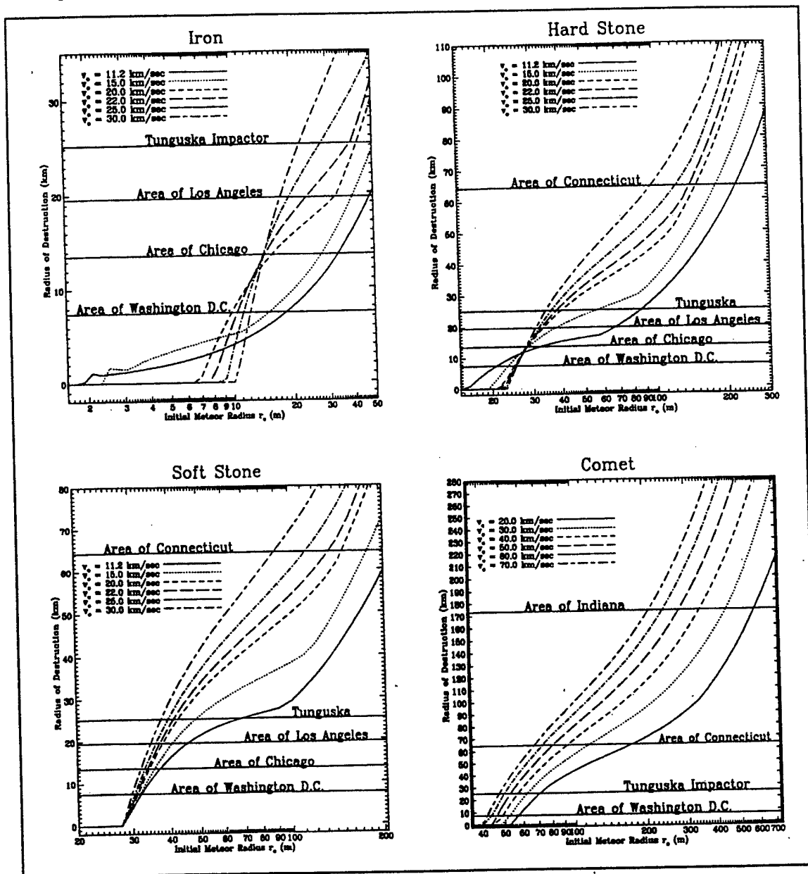
Figure 2.1 The radius of destruction around the impact point due to the atmospheric blast wave (from Hills, 1993, p. 1133).
