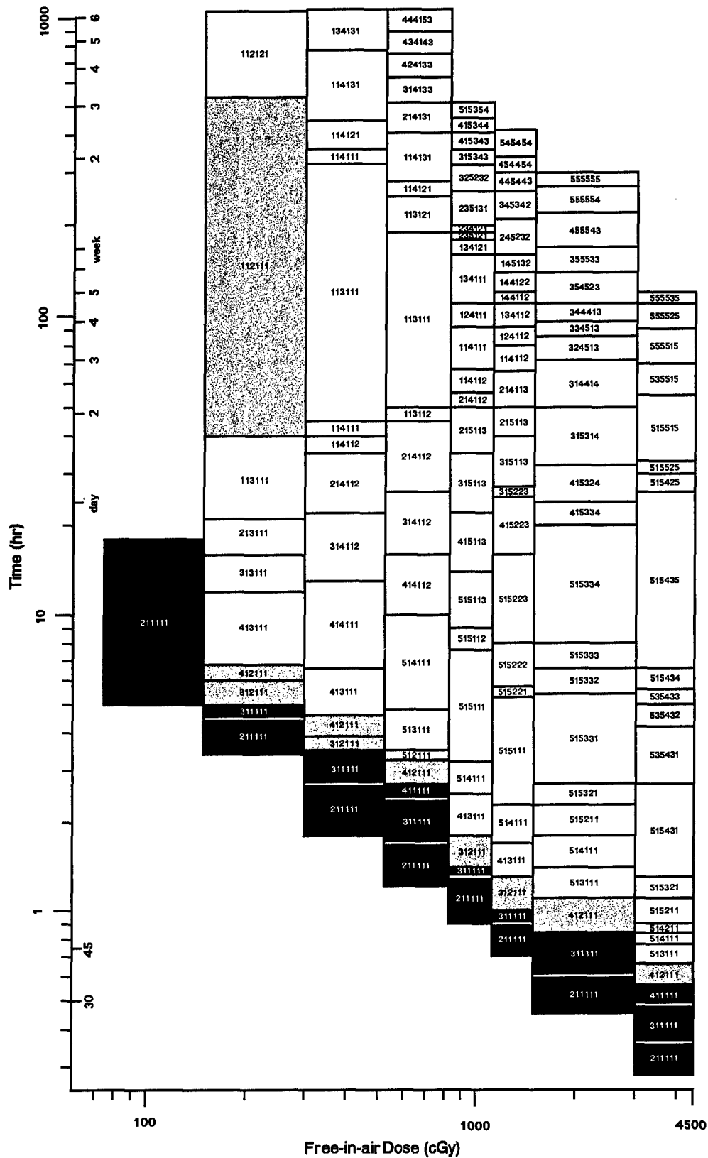
Fig. 5. Sign/symptom complexes for exposure to nuclear radiation—symptomatology map.
