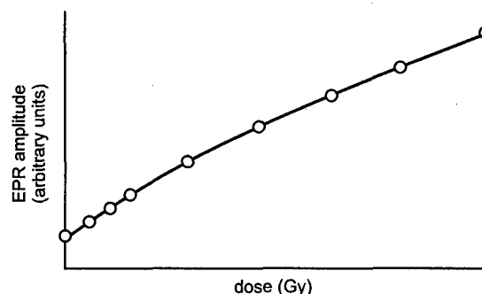
Fig. 18. Typical calibration curve for alanine dosimeters.
