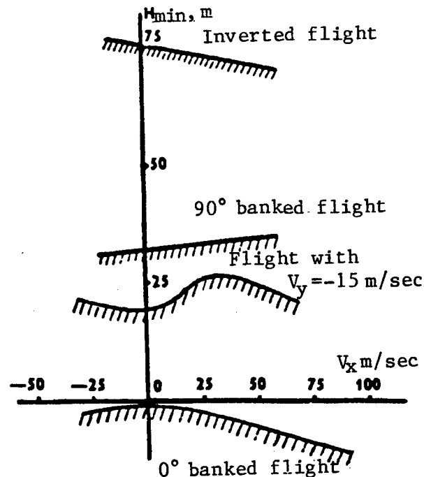
Lower limits of minimum heights H_{min} for rescue in various flight regimes
