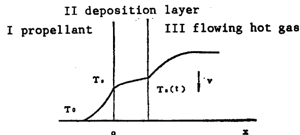
Figure 3. Surface Deposition Ignition Model
