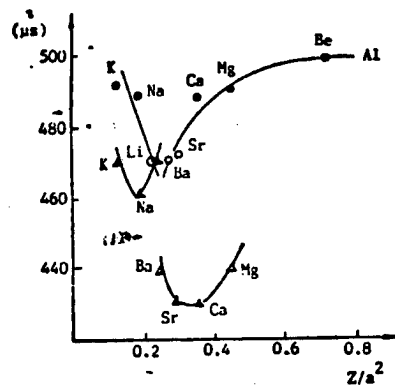
Fig. 5 Fluorescence lifetime of Nd^{3+} vs Z/a^2
