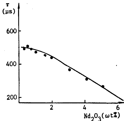
Figure 7. Concentration Quenching of \text{Nd}^{3+} -Fluorescence in Fluorophosphate Glass
