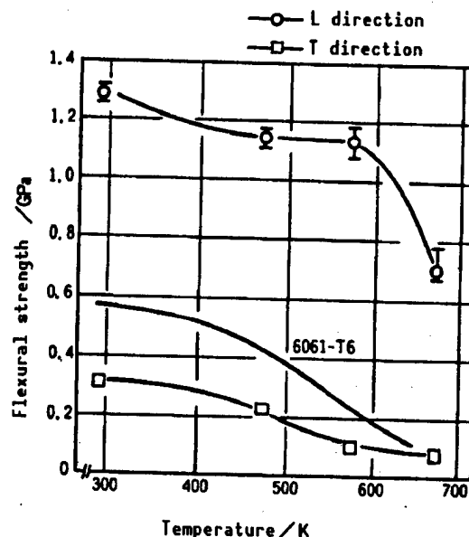
Figure 3. Effect of Temperature on the Flexural Strength of Tyranno Fiber-Reinforced Al
