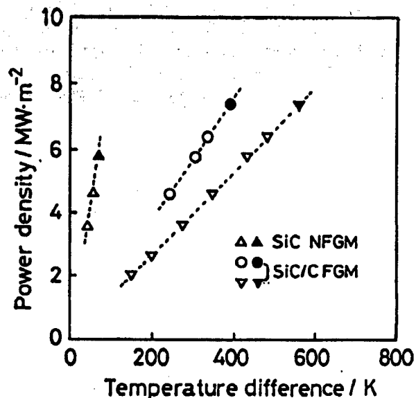
Figure 8. Relationship Between Laser Power Density and Calculated Temperature Difference in Thermal Shock Resistance Test (o: No cracking; \bullet : Cracking)
