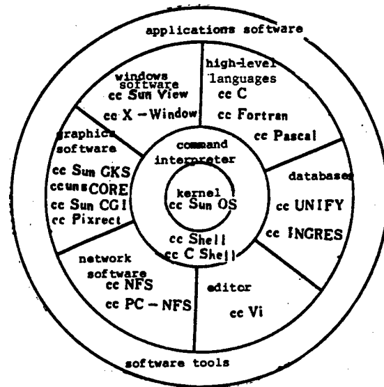
Figure 2. Software Levels for the Huasheng 3000 Series Workstations
