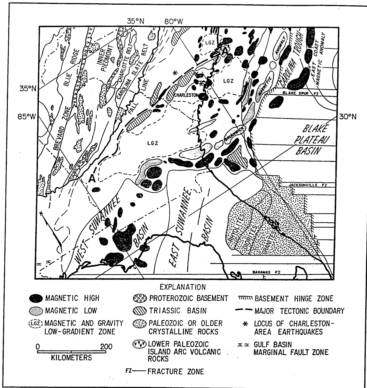
Figure 1. Geology and tectonism in the Charleston, South Carolina, region. From Klitgard et al. (1983).
