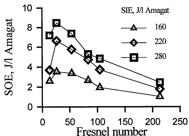
Fig.2.13. FO CO laser specific output energy vs. Fresnel number for thick filter CO : N 2 : He = 1 : 9 : 10; N = 0.3 Amagat; T = 100 K
