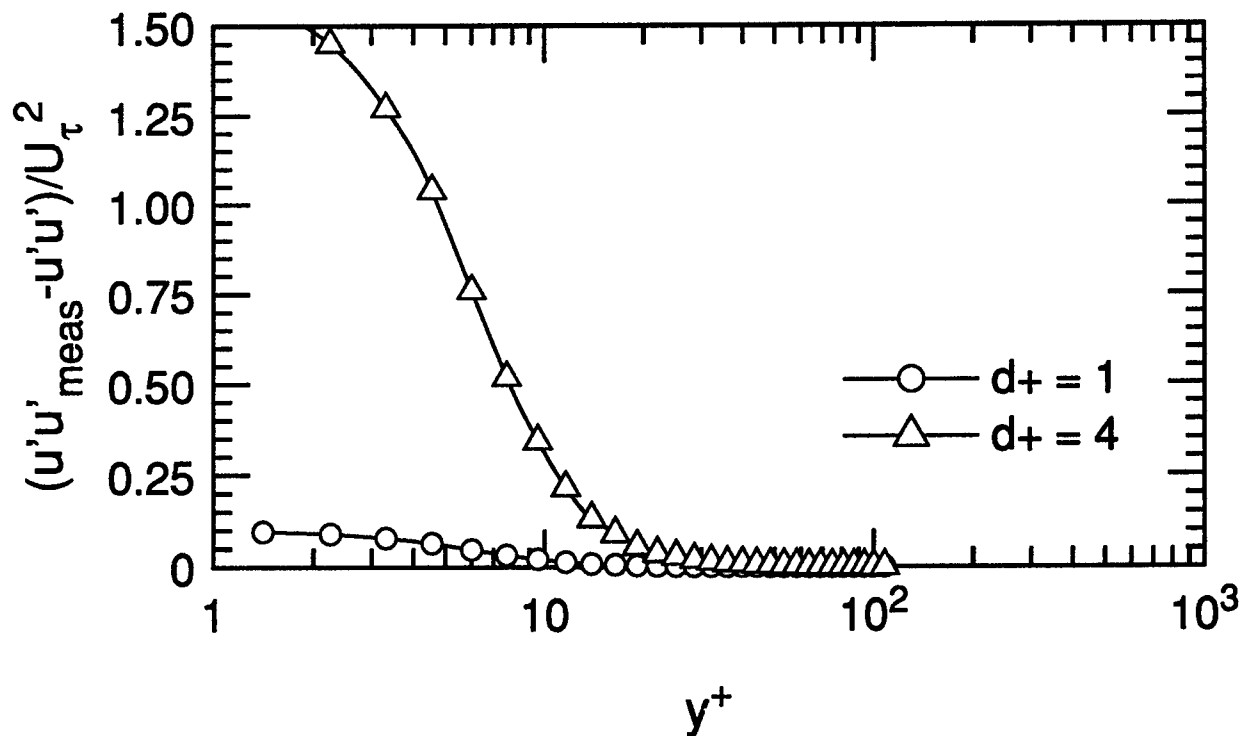
Figure C.2. Error in \overline{u'^2} due to finite volume size. Scaled on u_\tau .
