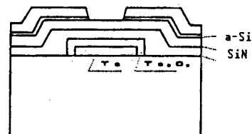
Figure 10. TFT Using \text{Ta}_2\text{O}_5/\text{SiN} Two-Layer Gate Insulating Film
