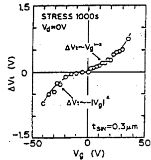
Figure 5. Drift Voltage
