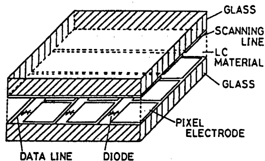
Figure 4. Structure of Diode LCD
