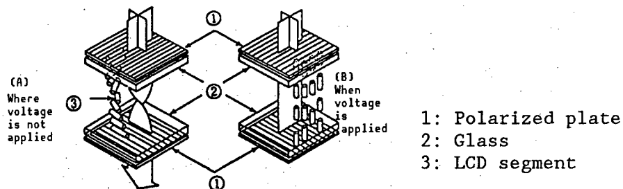
Figure 1. Operation Principle of TN System
