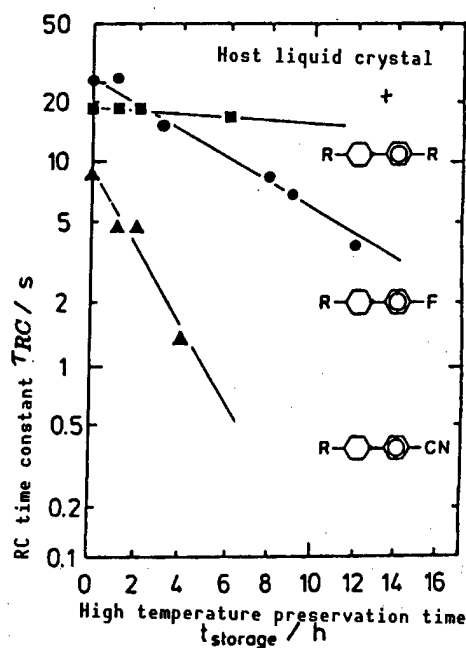
Figure 8. High Temperature Preservation Characteristic of Liquid Crystal Material
