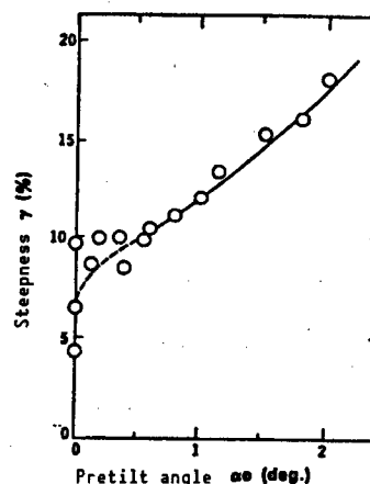
Figure 8. Relationship Between Pretilt Angle \alpha_0 and Steepness \gamma
