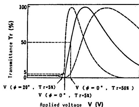
Figure 7. Tr-V Characteristic of VAN-Type LCD
