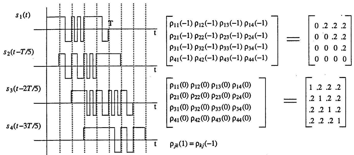
Figure 6a An example set of signature waveforms and delays which yield the correlation structure shown.
