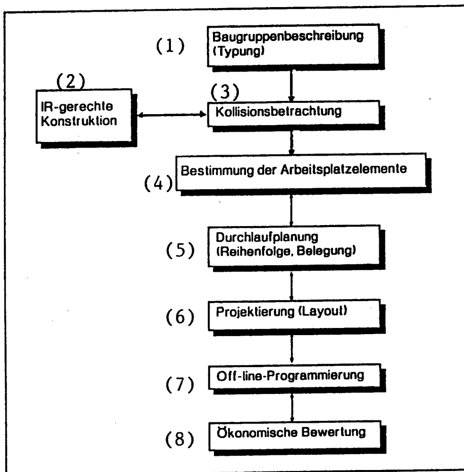
Figure 2. Comprehensive System for Rational Preparation for the Use of Industrial Robots for Welding of Large Assemblies
