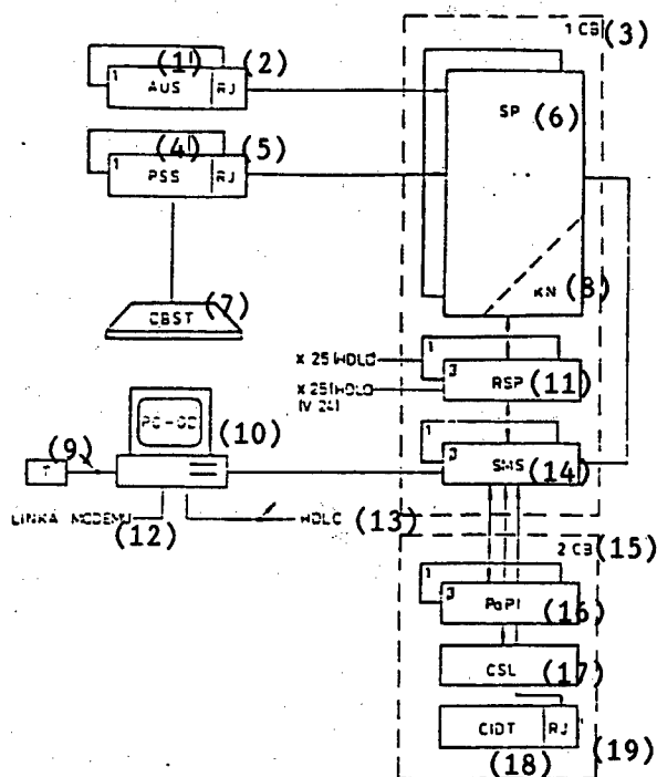
Figure 1. Block Diagram of UE 300 D System
