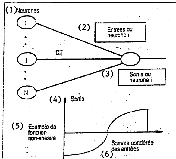
Figure 2. A neural circuit component, or "neuron", is a basic processor that performs two functions: storage of the network's synaptic coefficients, C_{ij} , acquired during the learning stage; and computation of output, which is a function of the weighted sum of the input data.
