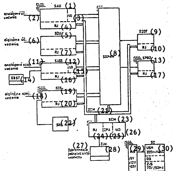
Figure 2. Block Diagram of UE 60 D PBX Exchange
