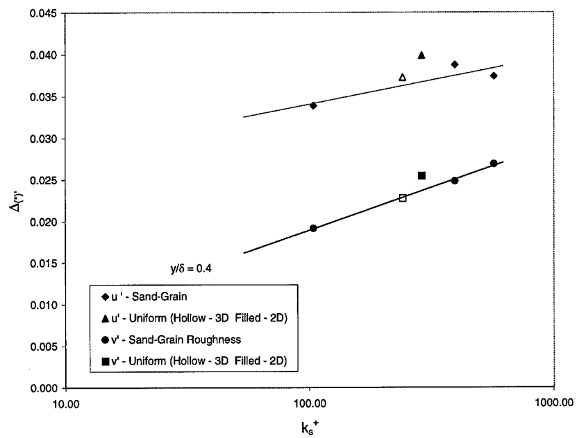
Figure 71. u - and v -Turbulence Intensity Versus Roughness Reynolds Number
