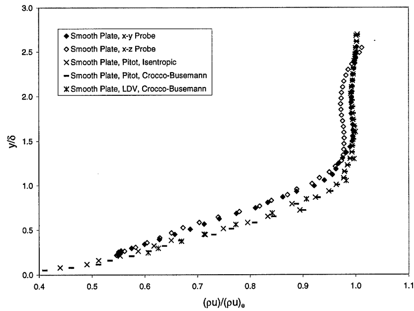
Figure 245. Smooth Plate (\rho u)_{\bar{a}r} Profiles
