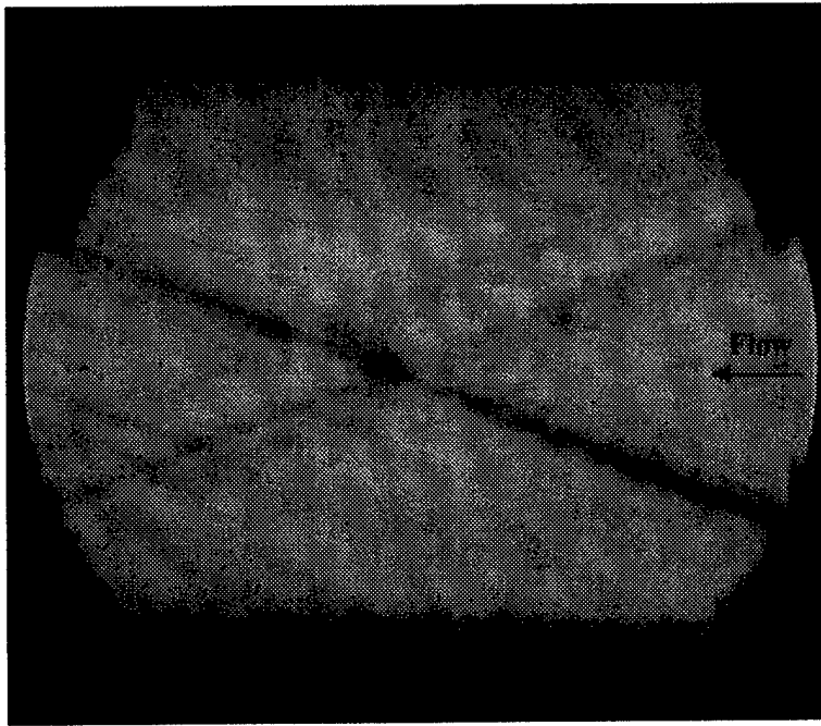
Figure 25. 3D Plate Schlieren at Nozzle Exit, Horizontal Knife Edge
