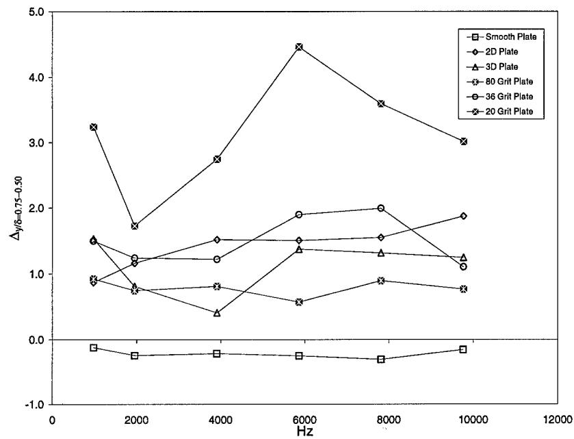
Figure 120. Power Spectra Difference, (\frac{p}{\delta})_{0.75} - (\frac{p}{\delta})_{0.50}
