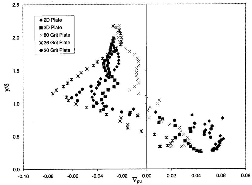
Figure 53. x - z Plane, Cross-Film, Rough Surface (\rho u)_{bar} Profiles Relative to Smooth Plate
