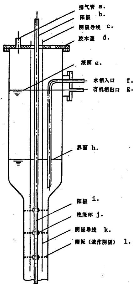
Figure 1. Simplified Diagram of Electropulse Column
