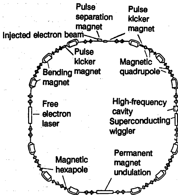
Figure 2. 800 MeV Electron Storage Ring
