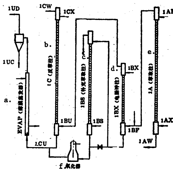
Figure 4. Simplified Diagram of Experimental Flow Process
