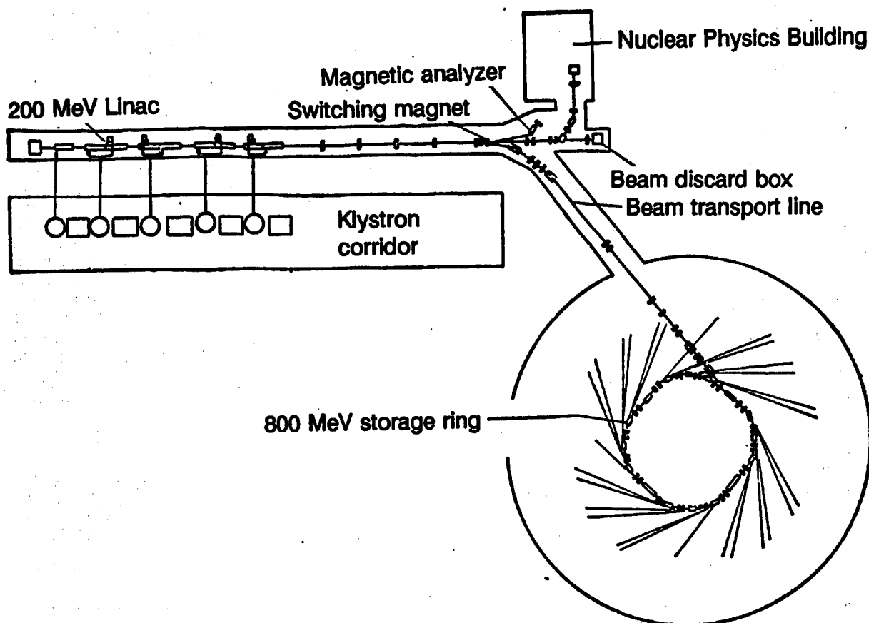
Figure 1. Layout of the Hefei National Synchrotron Radiation Source
