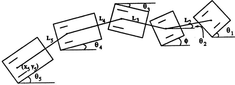
FIGURE 2. A 5-axle trailer system with the first two axles steerable.
