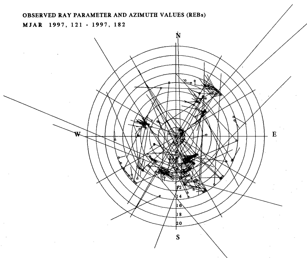
Fig. 7.7.1. Theoretical azimuth and ray-parameter values for the 294 onsets investigated are given by small circles. The corresponding values as reported by the PIDC in its final bulletins (REBs) are given as the end points of the lines.
