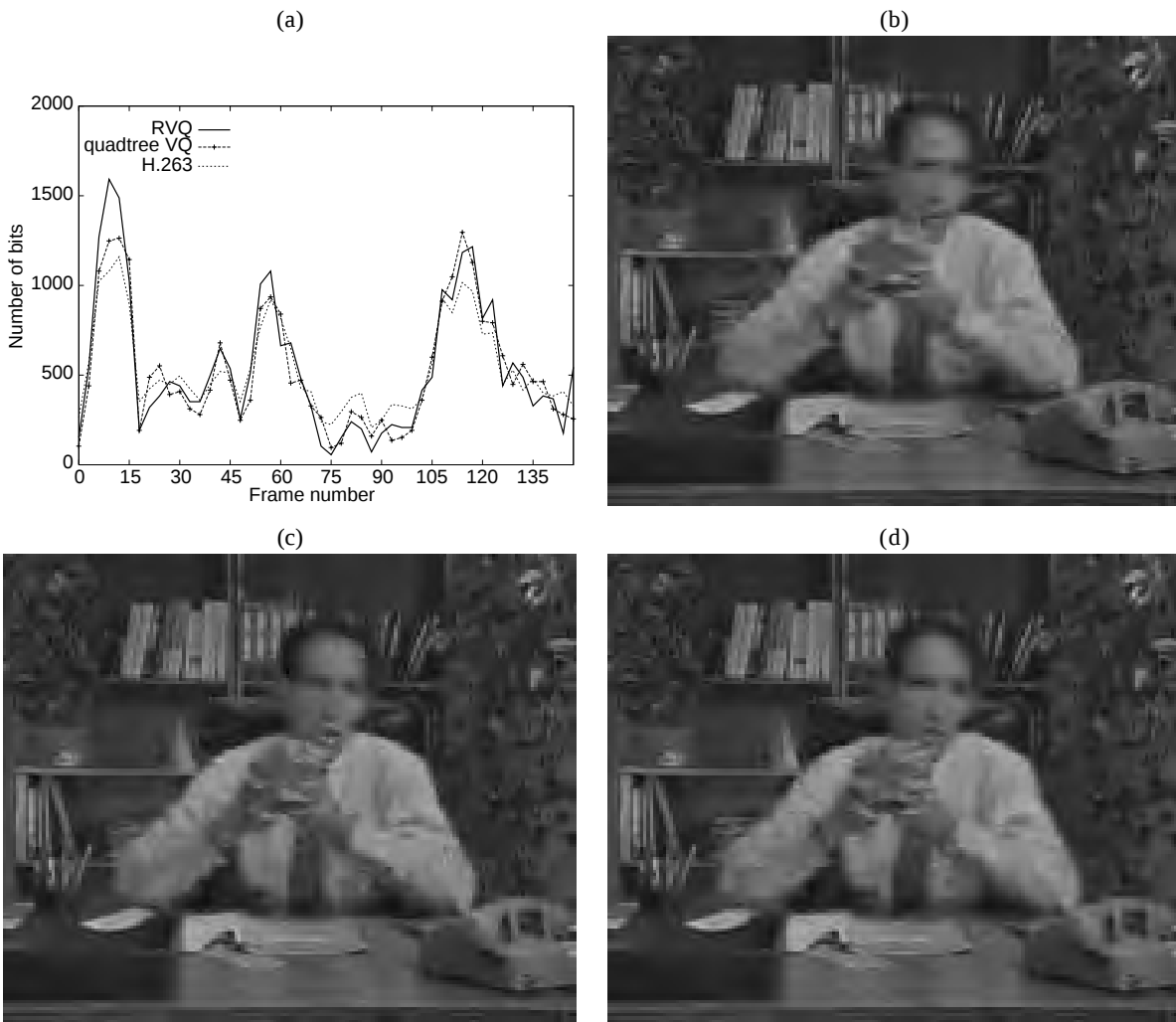
Figure 18. Results for bit rate of approximately 5.3 kb/s: (a) frame bit rate for sequence, (b) RVQ codec, (c) quadtree-VQ codec, and (d) H.263 codec.
