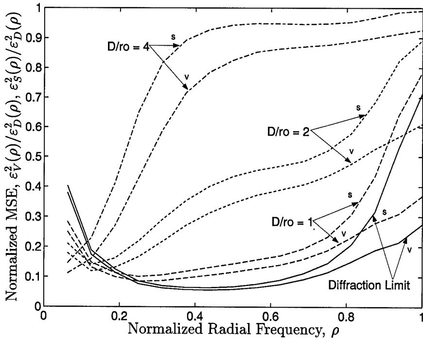
Figure 5.17 Normalized MSE, \epsilon_V^2(\rho)/\epsilon_D^2(\rho) and \epsilon_S^2(\rho)/\epsilon_D^2(\rho) , for the diffraction-limited OTF and D/r_o = 1, 2, and 4 ( \bar{K} = 500 photoevents). The v and s designators differentiate between vector and scalar Wiener filter traces.
