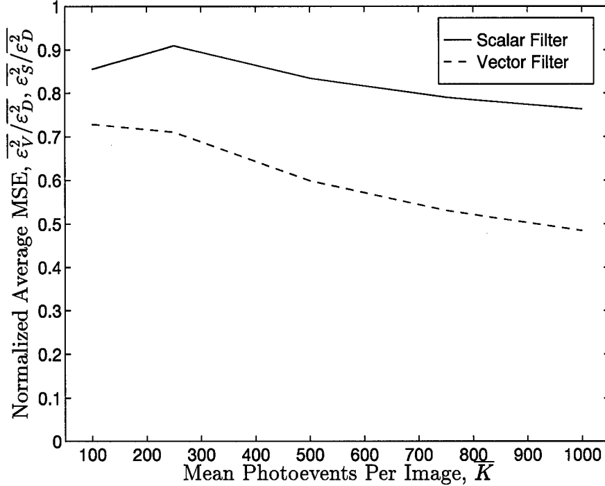
Figure 5.7 Normalized average MSE, \overline{\varepsilon_V^2}/\overline{\varepsilon_D^2} and \overline{\varepsilon_S^2}/\overline{\varepsilon_D^2} , versus \bar{K} . Support constraint dimension W = 8 pixels and pupil size D_p = 6 pixels.
