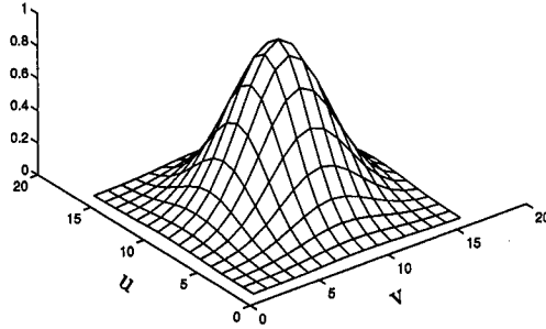
Figure 6.2 Mesh plot showing the mean OTF, \bar{\mathcal{H}}(u, v) , for mean OTF width parameter, w_{\mathcal{H}} = 0.5 .
