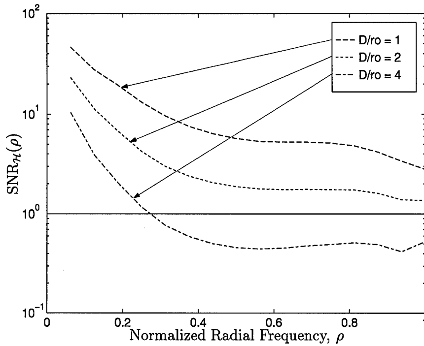
Figure 5.13 Tilt-removed OTF SNR, SNR_{\mathcal{H}}(\rho) , due to atmospheric turbulence versus radially averaged spatial frequency \rho (von Karman turbulence statistics L_o/r_o = 100 , D/r_o = 1, 2 , and 4 ). Note that SNR_{\mathcal{H}}(\rho) < 1 when \rho > 0.3 in the D/r_o = 4 case.
