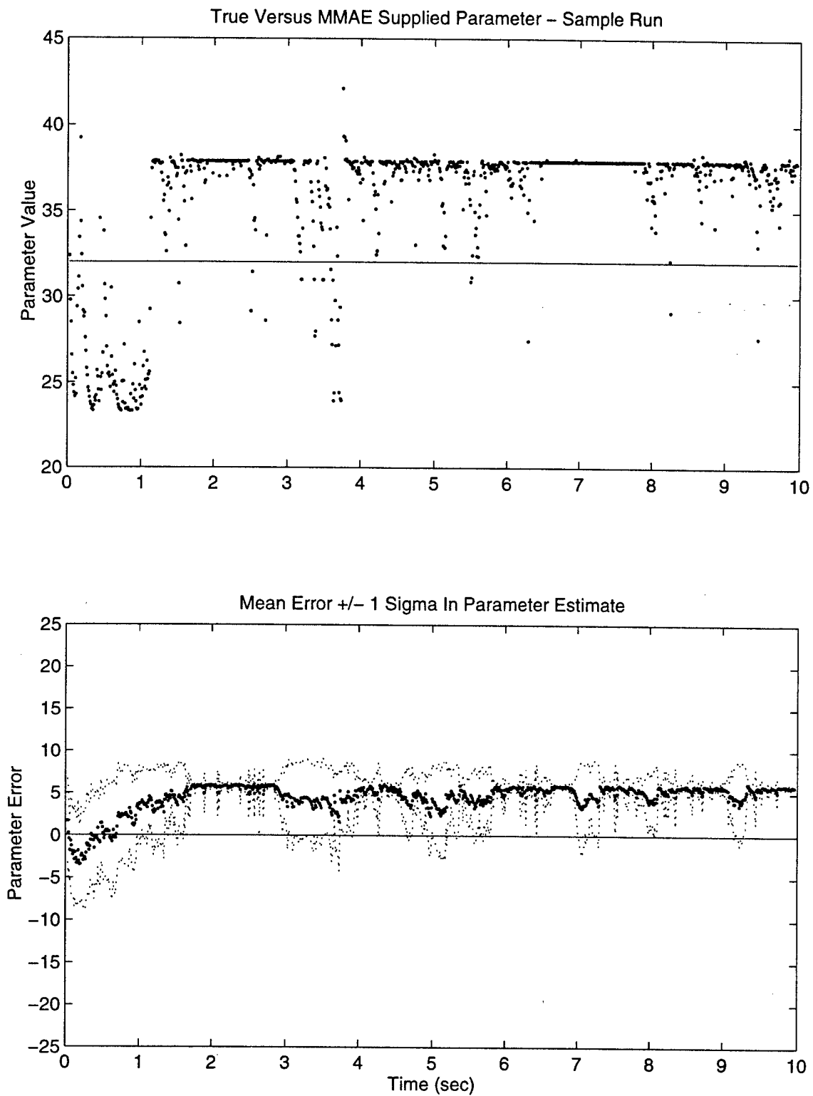
Figure 30. MMAE/SDSEP Parameter Estimation Performance: Test Case 1
