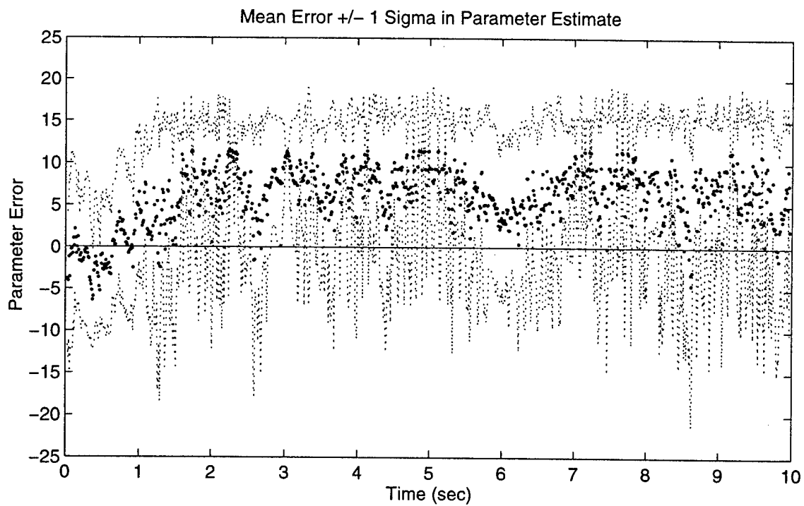
Figure 38. MMAE/SDPEP With IRDF Parameter Estimation Performance: Test Case 2
