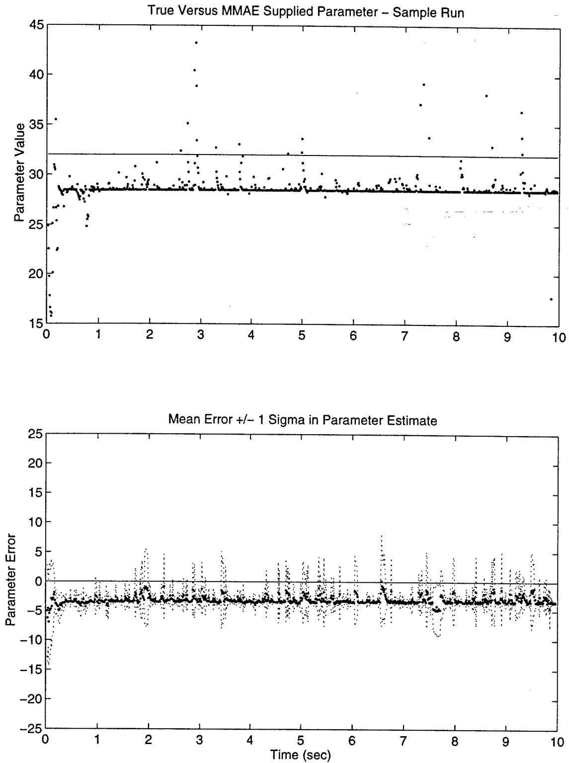
Figure 15. MMAE/SDPEP Without IRDF Parameter Estimation Performance: Test Case 1
