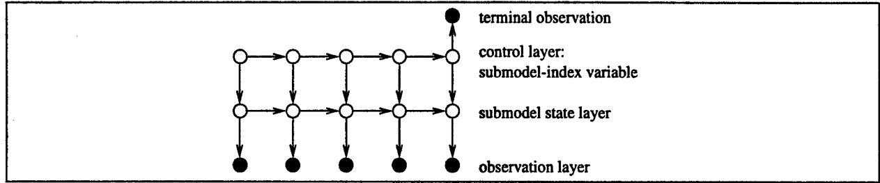
Figure 4: A DPN structured for model composition. The submodel-index variable specifies which submodel to use at each point in time.
