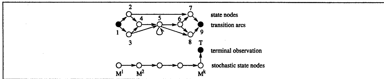
Figure 3: An SFSA and a DPN network representation for fixed-length observation sequences. Note that in the automaton the arcs represent transition probabilities while in the probabilistic network they represent conditional independence relations. The initial and final states of the SFSA are shaded. The shaded node in the DPN represents an artificial observation; the CPT of this variable will encode the length of the observation sequence.
