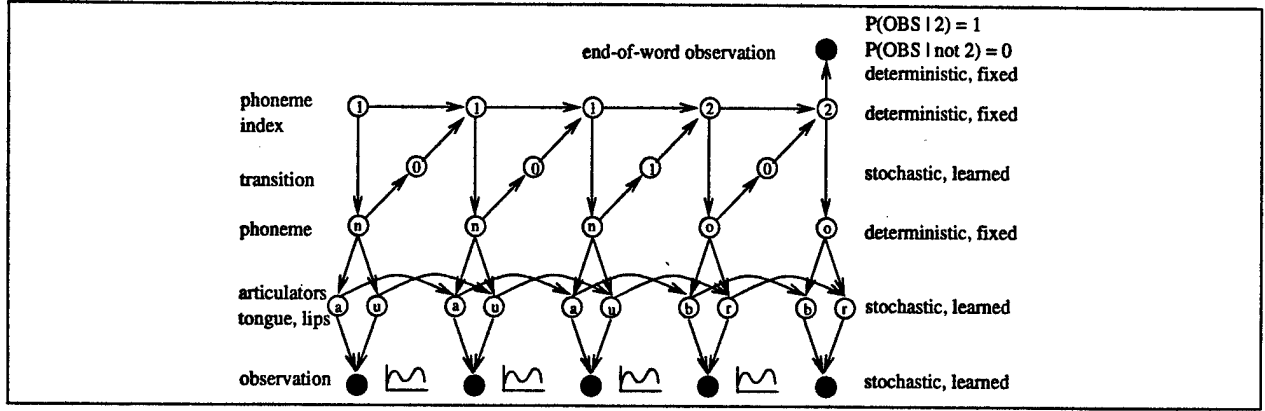
Figure 5: A DPN structured for speech recognition. The unshaded variables are hidden, and the labels attached represent just one acceptable assignment of values to them. The tongue moves from the alveolar ridge to the back of the mouth; the lips move from an unrounded to a rounded configuration. The properties of each node are shown to the right. Nodes whose CPTs are fixed are fixed on a per-example basis.
