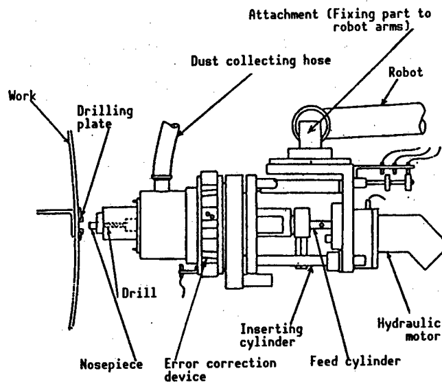
Figure 3. Drilling Head
