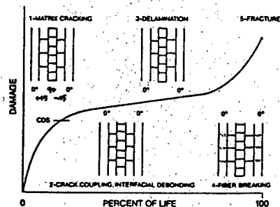
Figure 11. Process of Fatigue Damage in Multilayer Laminates 8
