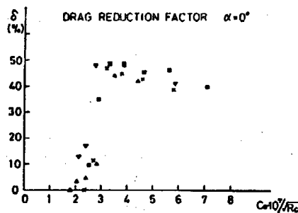
Figure 10. Drag Reduction Factor
