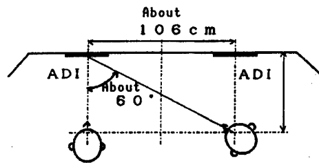
Figure 9. Facing Angle of Captain Seat ADI From Co-Pilot Seat (Case of large transport planes)
