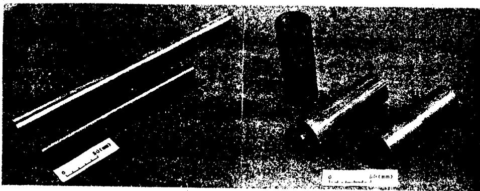
Figure 6. External Appearance of Samples of Trial Manufactured Tube-Shaped FRMs
