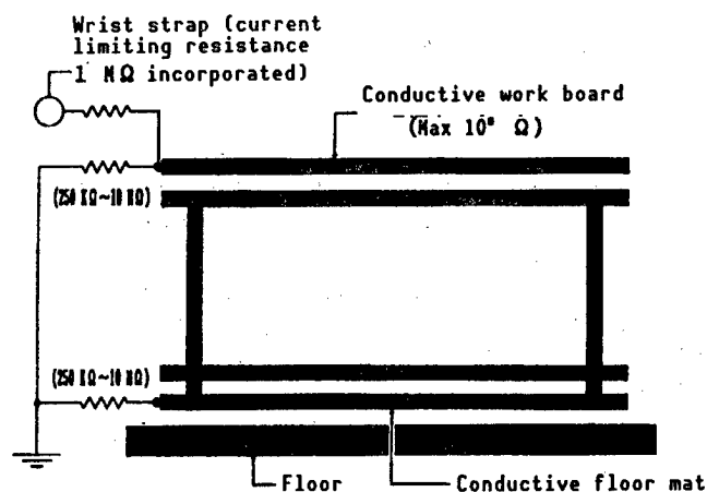
Figure 4. Workbench
