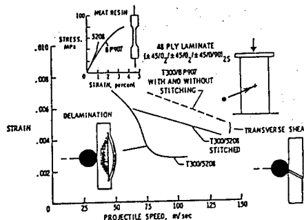
Figure 10. Effects of Improved Toughness of Resins and Stitching on the CAI Characteristic 7
