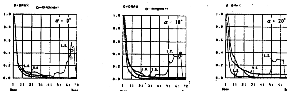
Figure 5. Aerodynamic Heating Distribution of SPH002 Surroundings ( M_\infty = 7.0 , Re_\infty = 4.4 \times 10^6 )
