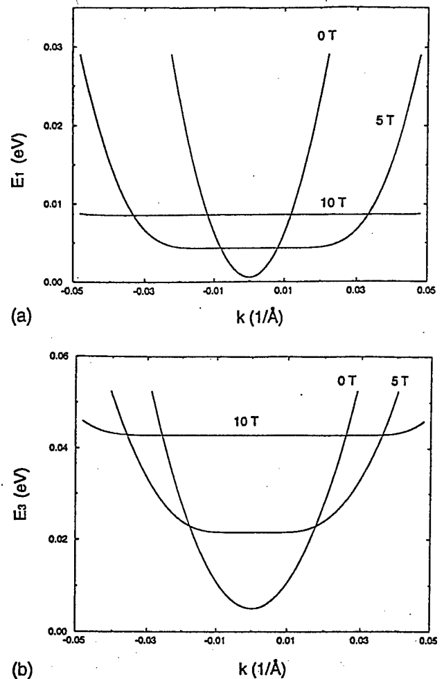
FIG. 4. Energy vs wave vector relation of electrons in (a) the first subband and (b) in the third subband of a 1000 \text{ \AA} wide quantum wire. The wave vector is along the free propagation direction. The results are shown for three values of a magnetic field. The energy is calculated from the bulk conduction band edge and the confinement energy for the z -direction is assumed to be zero.
