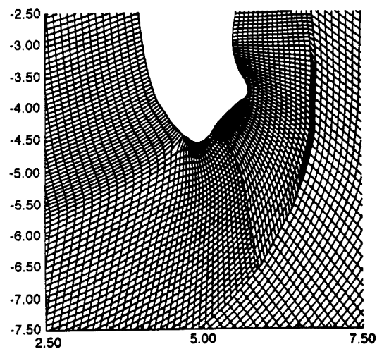
Fig. 15. Deformed mesh of the ejecta of the WHA rod at t = 22.5 \mu s .
