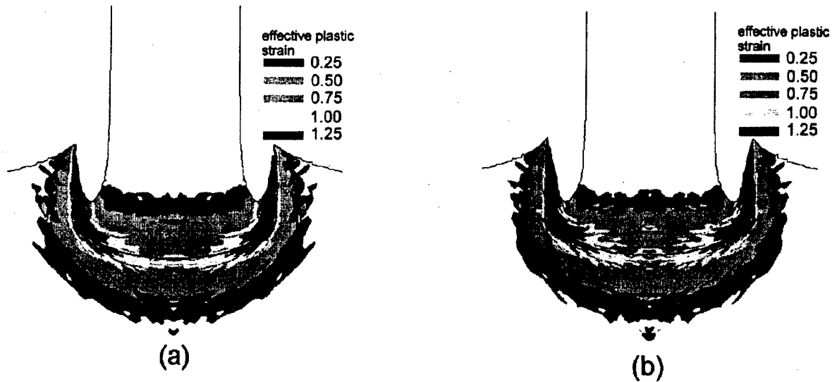
Fig. 13. Fringes of effective plastic strain at time, t = 10 \mu s for (a) DU; (b) WHA penetrator.
