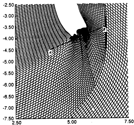
Fig. 14a. Deformed mesh of the ejecta of the DU rod at t = 22.5 \mu s , and the location of line AB on which the effective plastic strain is plotted in Fig. 14b.
