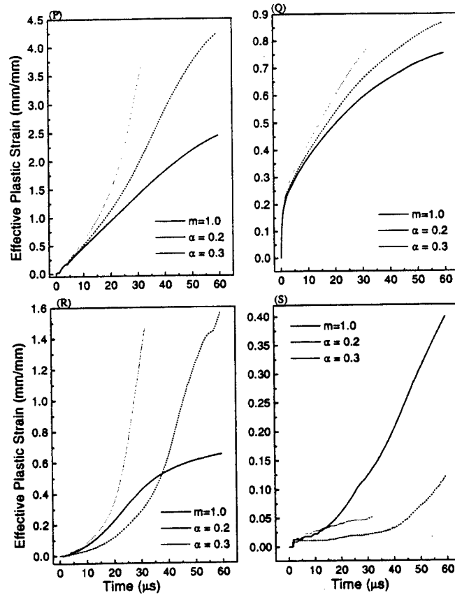
Fig. 10. Time history of effective plastic strain in elements in the WHA rod located at points p , Q , R and S .
