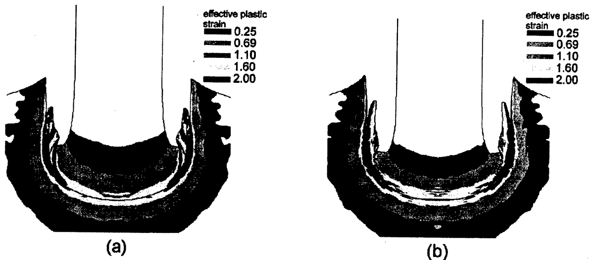
Fig. 14. Fringes of effective plastic strain at time, t = 20 \mu s for (a) DU, (b) WHA penetrator.
