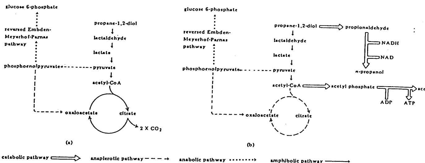
SCHEME I. Pathways of (a) aerobic and (b) microaerophilic metabolism of propane-1,2-diol by Flavobacterium sp NCIB 11171.
