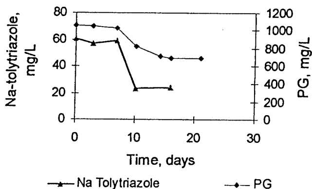
Figure 12. Na Tolytriazole Degradation
