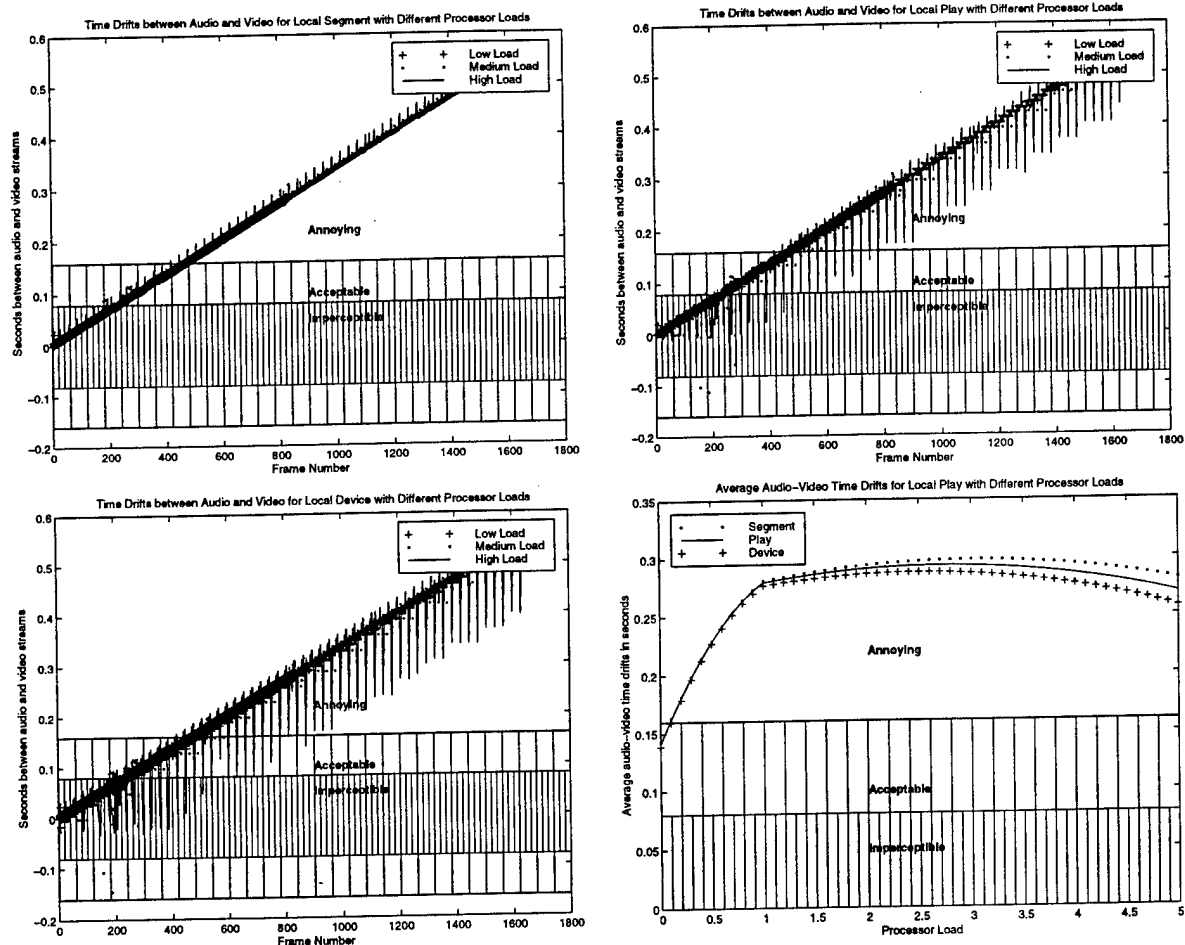
Figure 3: Synchronization Behavior of Local Playback
