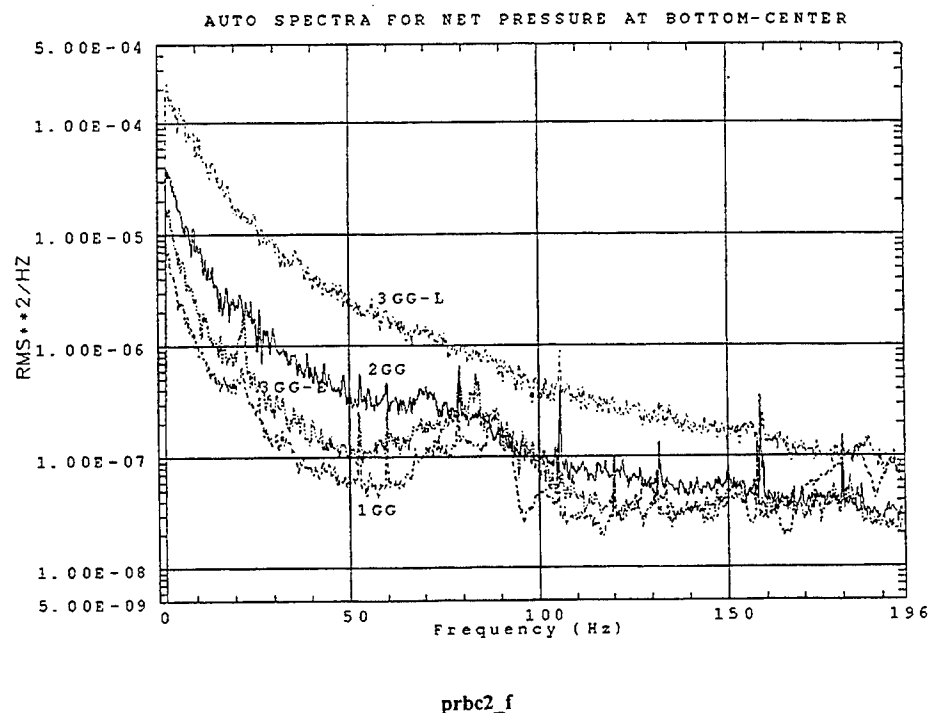
k. Net pressure at bottom center on gate
