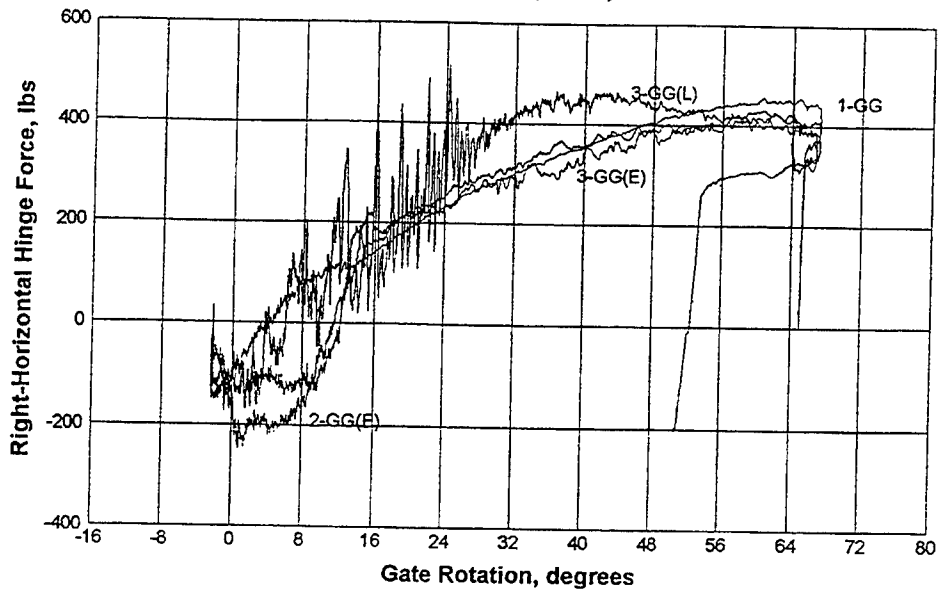
c. Right horizontal hinge load
