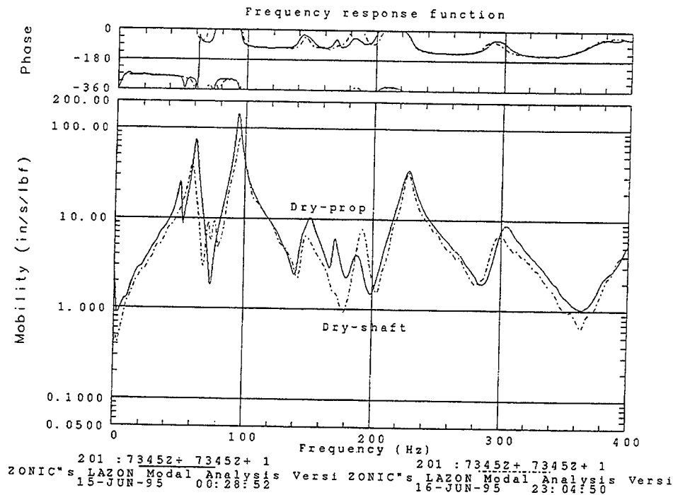
Figure 101. Mobility response function comparision for prop- and shaft-supported dry wickets
