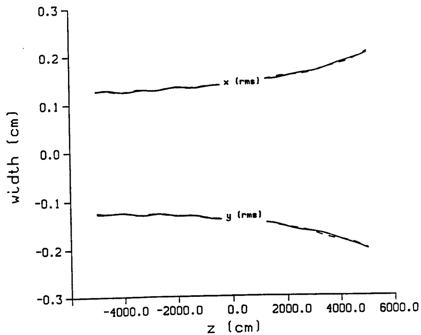
size of electron beam
