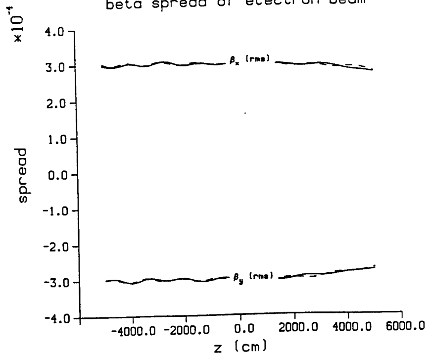
beta spread of electron beam
