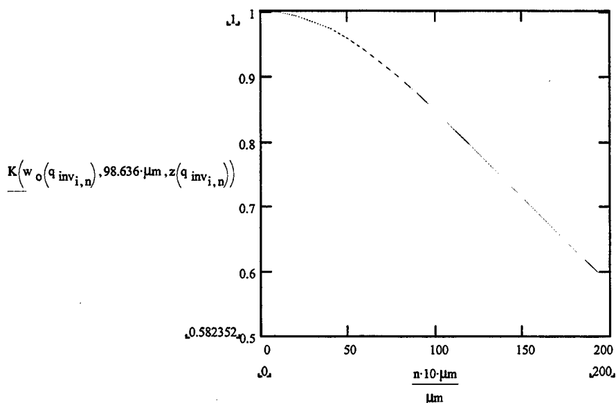
Figure 6 The change in normalized coupling efficiency in a previously optimized System A as the GRIN is polished back.
