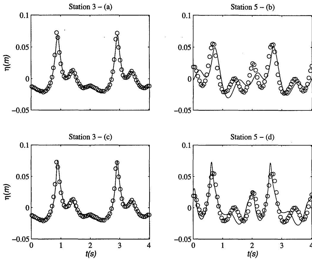
Figure 6.13: Comparisons of free surface displacement with case (4) of the Ohyama experimental data at stations 3 and 5. FN4 (upper panels - a,b), WKGS (lower panels c,d), data (circles).
