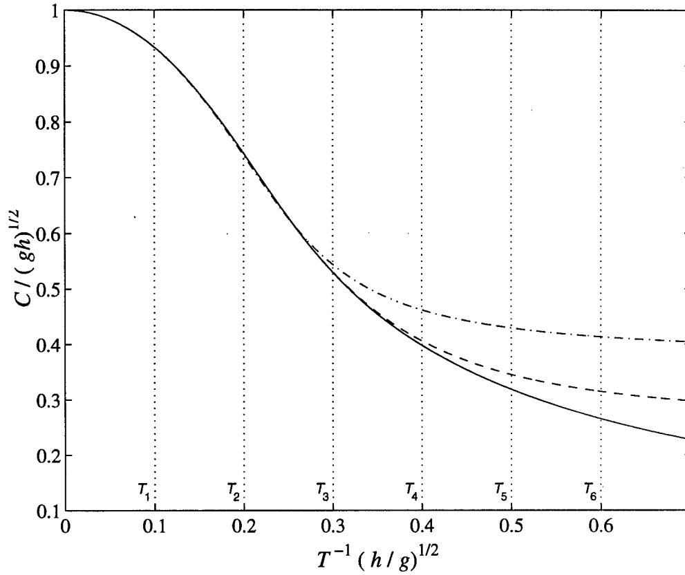
Figure 6.4: Linear dispersion relationship as (nondimensional) wave speed vs. wave frequency. Present Model (dash), WKGS (dash-dot), exact (solid). Dotted vertical lines are waves with periods T_n = (2.02/n)s .
