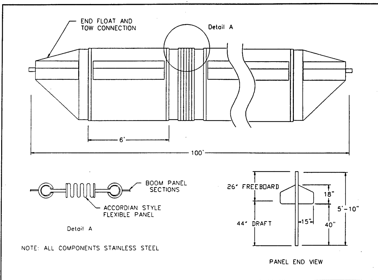
Figure 2 Details of the Dome Boom
