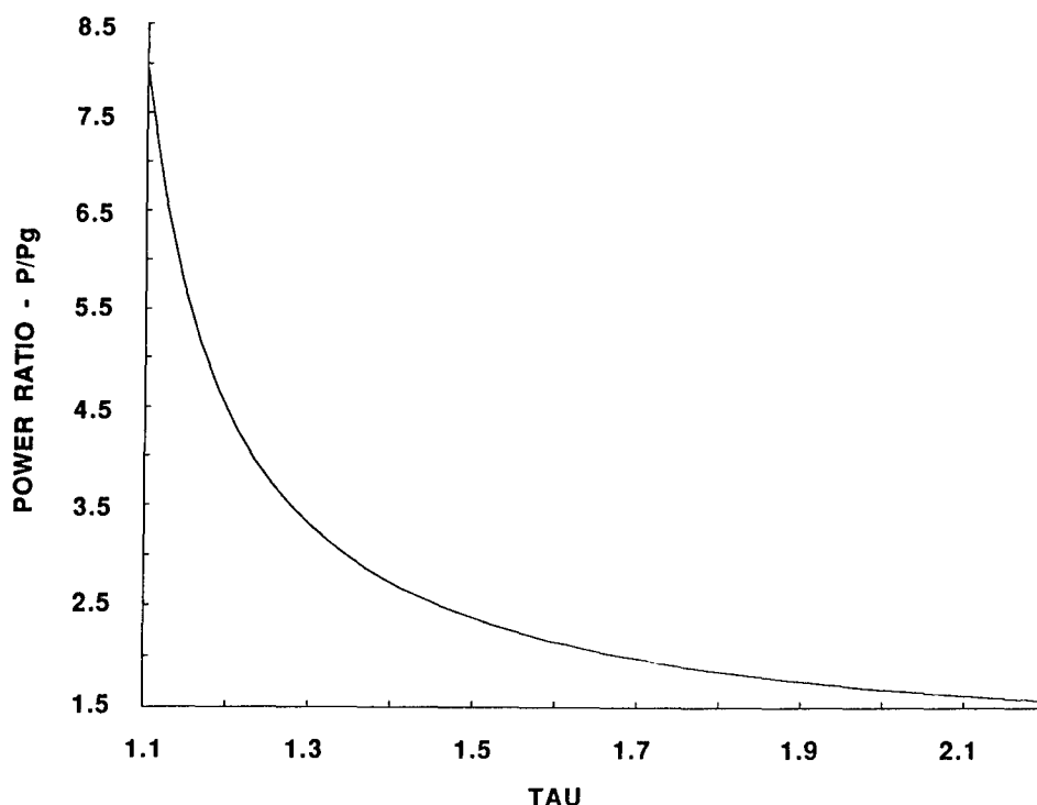
Figure 6: Power ratio versus tau.
