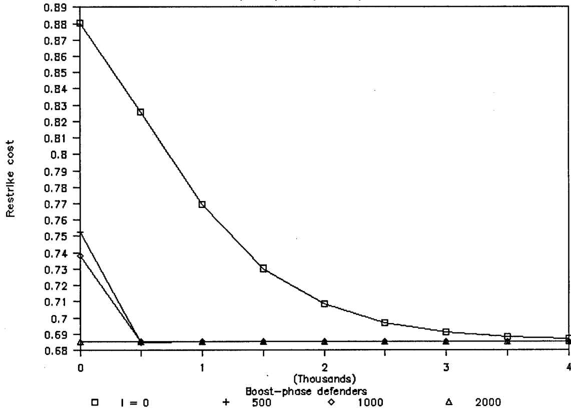
Fig. 13 Restrike cost
