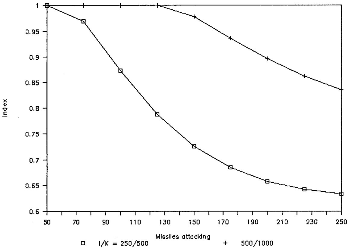
Fig. 22 Stability index
