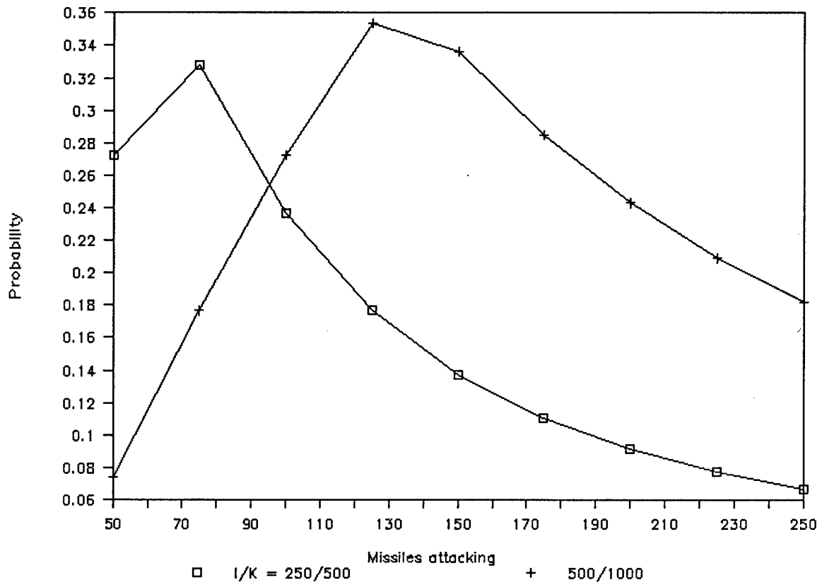
Fig. 17 Survival/pen. probability
