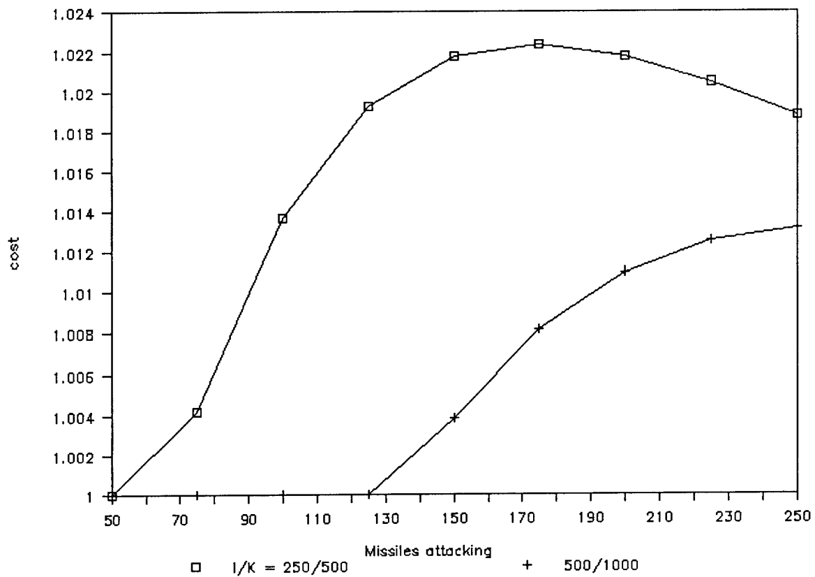
Fig. 27 Stability index
