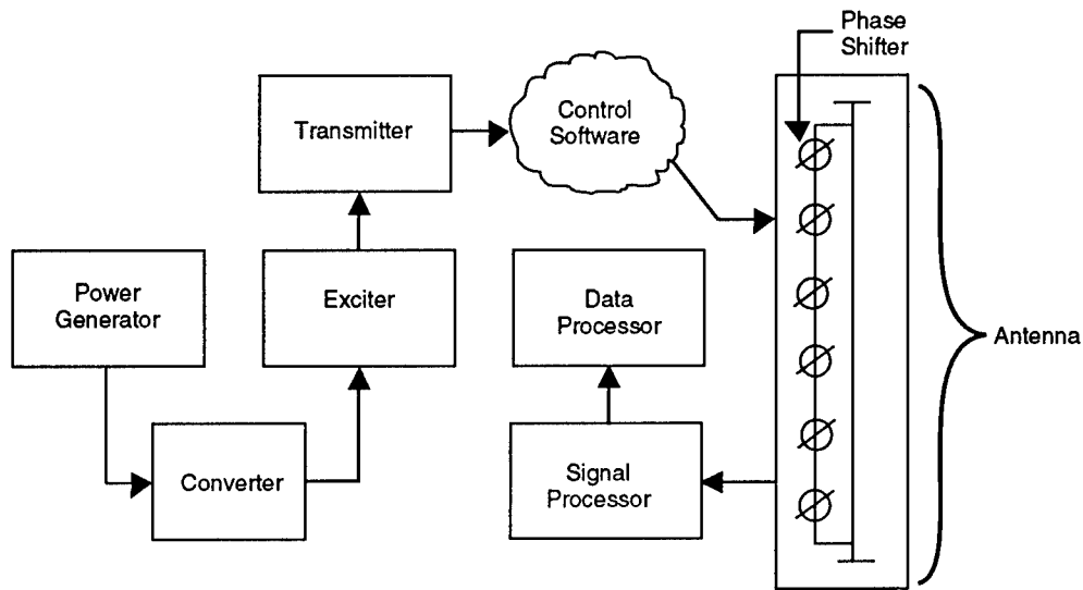
Figure 5.3: GBR Components
