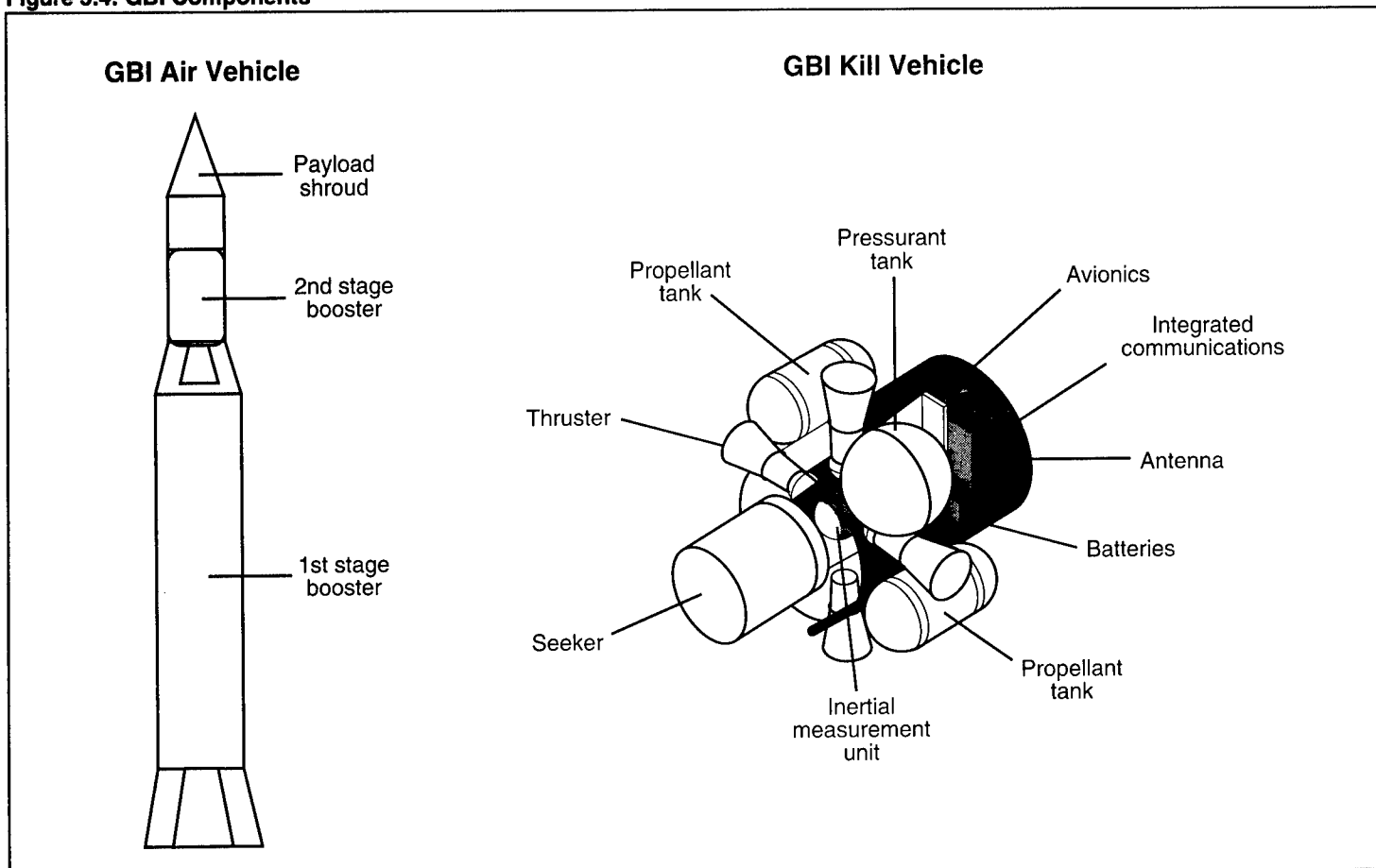
Figure 5.4: GBI Components
