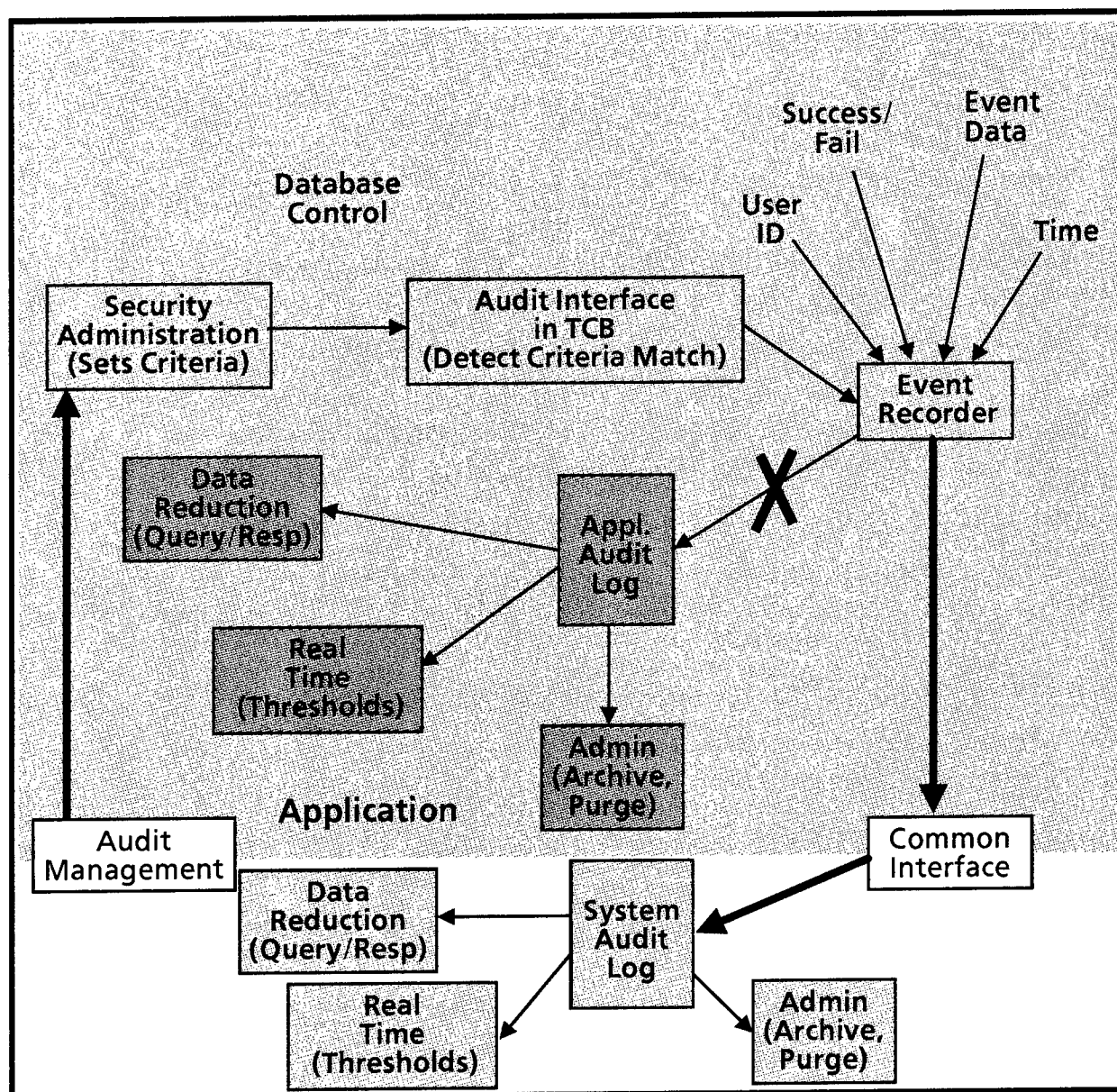
Figure 3. Centralized Audit Administration
