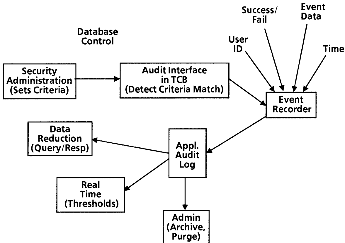
Figure 2. An Example Application's Audit Function
