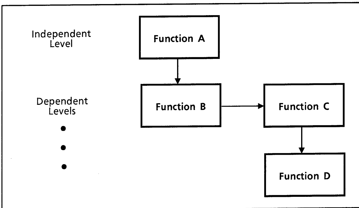
Figure 1. Dependency Lattice
