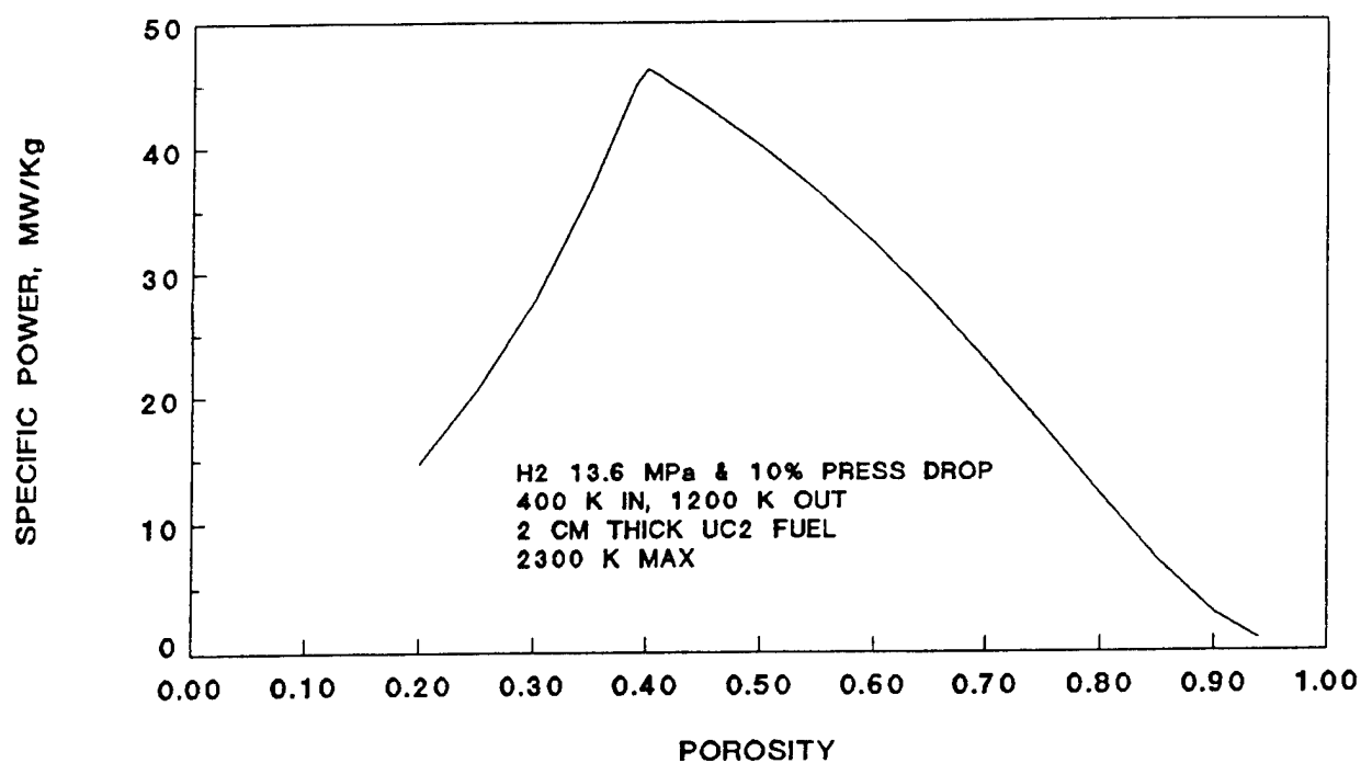
Figure C-11. Specific Power of Foam-Fuel Reactor Burst Mode
