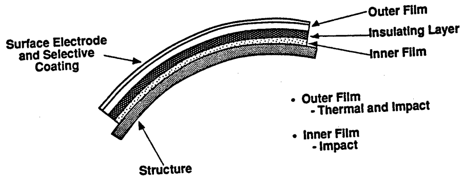
Figure 5. Schematic of Polymer Laser Sensor Skin.
