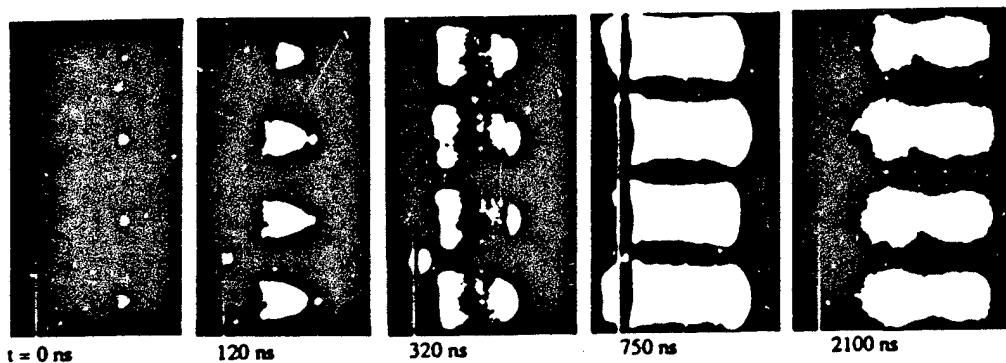
Figure 6: Side view of breakdowns above a row of 1.5 mm \phi /1 dimples at various times from start of laser pulse. Bright line is plane of dimpled surface; bright areas behind surface are reflections. Small specks are computer-generated fiducials. Laser pulse (1 \mu s, 4 J/cm 2 ) enters from right.
