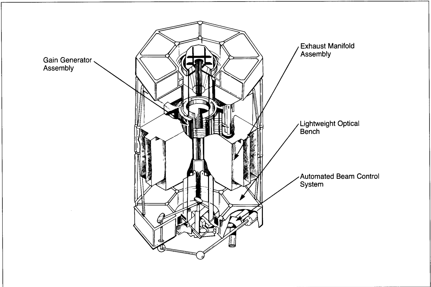
Figure 2.1: Illustration of the Alpha Laser
