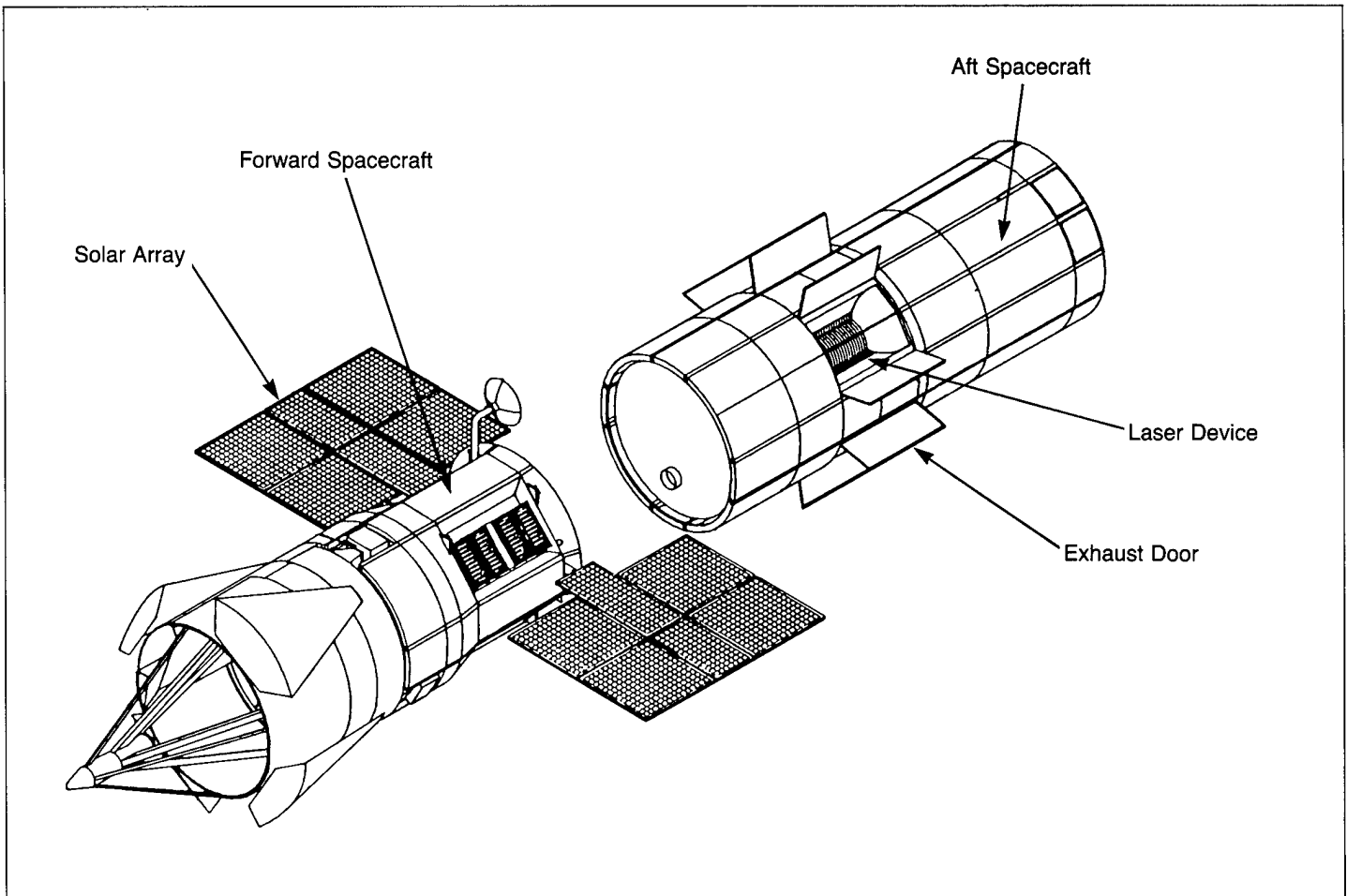
Figure 1.1: Zenith Star Forward and Aft Spacecraft
